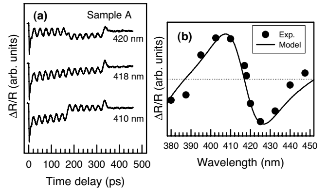
FIG. 4. (a) Reflectivity measurements obtained in sample A for three different laser wavelengths. One should remark the sign change in the reflectivity jump detected at 180 ps. (b) A comparison between the magnitude of the reflectivity jump detected in sample A as a function of the laser wavelength between experimental values and the theoretical model developed in the text. The excellent agreement has been obtained by fitting the \text{SiO}_2 thickness.
