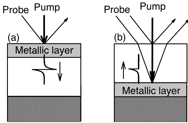
FIG. 1. Schematic diagram of the experiment. The pump light pulse generates a longitudinal acoustic pulse in the metallic layer. (a) The generation acts at the free surface and a bipolar shape strain pulse results. This is the usual case when a transducer is deposited onto the sample surface. (b) The metallic layer is buried so that the strain pulse which propagates in the transparent layer is monopolar (purely compressive). The probe beam causes interferences in the transparent layer as in a Fabry-Pérot interferometer.
