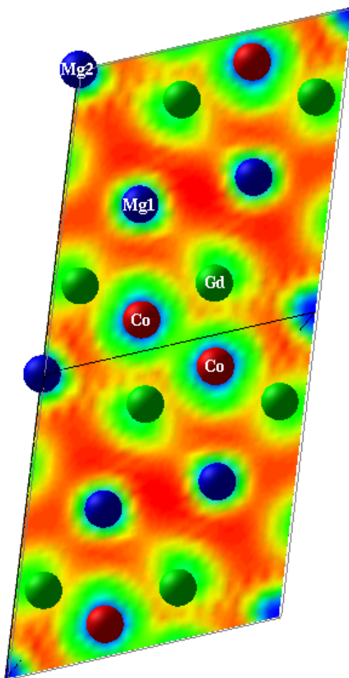
Fig. 3 (Color plot in the online version). ELF (electron localization function) contour plot for Gd_4Co_2Mg_3 (projected view of the x, 0, z basal plane (2 unit cells) containing the Mg1, Mg2 (blue spheres) and Co atoms; the Gd atoms (green spheres) are above the plane). The electron localization between Co atoms is free electron-like. Blue, green and red contours are for zero localization, free electron-like and full localization, respectively.
