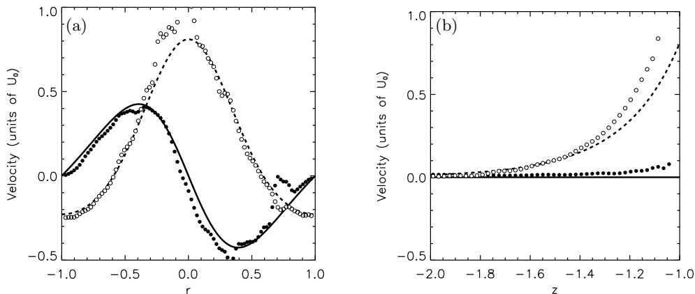
FIGURE 7. Comparison between theoretical and experimental velocity profiles, in units of U_0 in the confined geometry ( \lambda = 1 ). (a): the profile is taken along a ray tangent to the meniscus. (b): the profile is plotted along the symmetry axis. In both cases, the thick (dotted) line correspond to the radial (axial) theoretical velocity. The filled (empty) circles represent an experimental observation made with water, in a 3 cm diameter glass tube. The impact velocity is 6 m/s.
