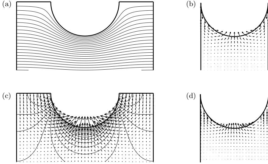
FIGURE 5. Left: pressure levels (a) and velocity field (c) obtained with the cylindrical representation for a value of the confinement factor of \lambda = 0.5 . (a) : the isobars are equispaced with a step of 0.08\rho U_0 R . (c) : along with the velocity vectors are represented the levels of the pressure gradient norm. These are equispaced with a step of 0.12\rho U_0 . Right: the theoretical velocity field for the confined geometry ( \lambda = 1 ) is represented figure (b), whereas a typical velocity field obtained experimentally after PIV treatment is plotted figure (d).
