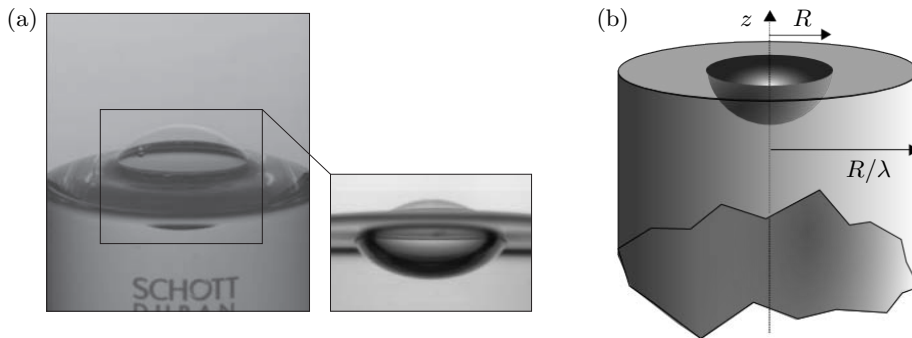
FIGURE 4. Left: Typical experiment of a cavity produced with a bubble, just before impact. Right: sketch of the liquid domain in the theoretical idealization.
