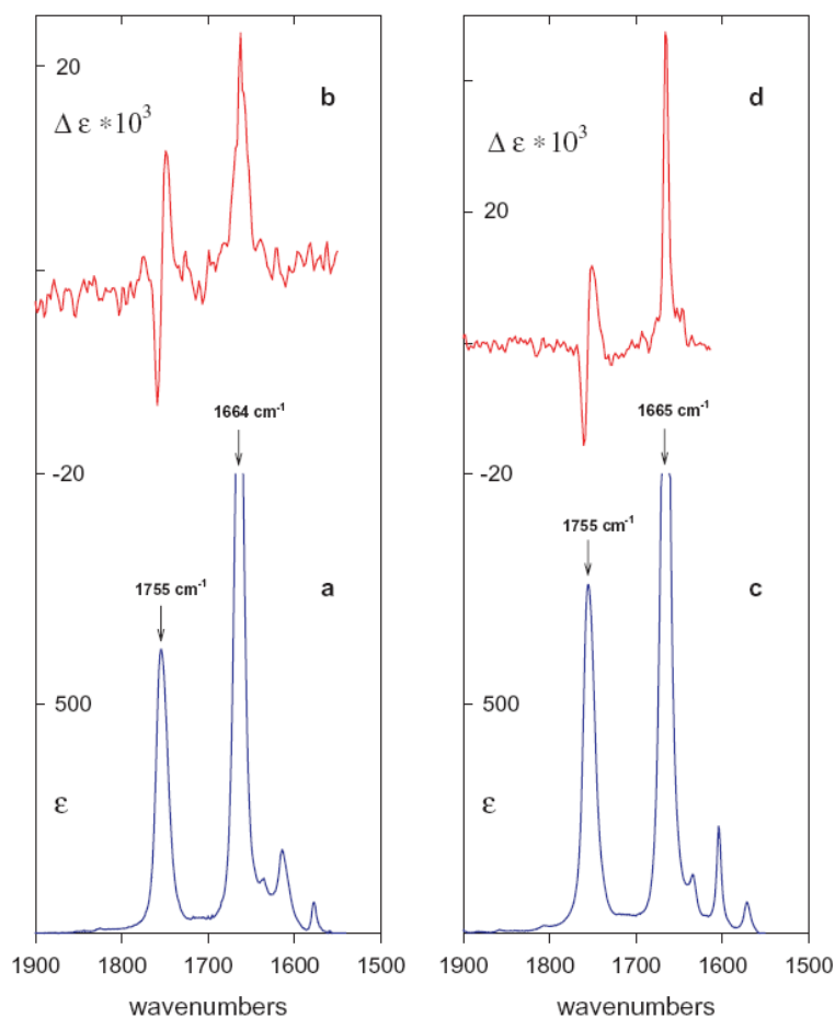
Figure 1. Experimental IR and VCD spectra of 3 and 4 in \text{CCl}_4 solution in the \text{C}=\text{O} stretching region. (a) IR: (–)- 3 , (b) VCD: (+)- 3 , (c) IR: (–)- 4 , (d) VCD: (+)- 4 .
