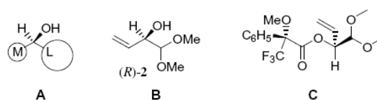
Figure 1. (A) Kazlauskas' model; M: medium substituent; L: large substituent. (B) ( R )- 2 corresponding to the model. (C) Mosher's ester of 2 .
