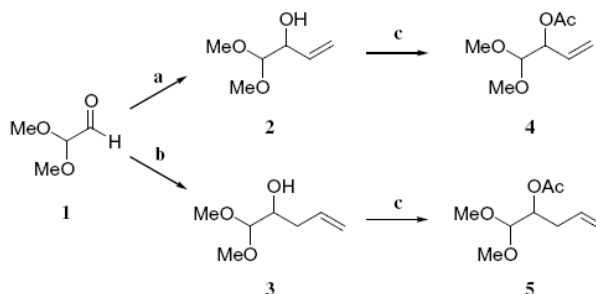
Scheme 1. Reagents: (a) \text{CH}_2=\text{CH}-\text{MgBr} , THF; (b) \text{CH}_2=\text{CH}-\text{CH}_2-\text{MgBr} , In, \text{H}_2\text{O} or \text{CH}_2=\text{CH}-\text{CH}_2-\text{MgBr} , THF; (c) \text{Ac}_2\text{O} , DMAP, pyridine.
