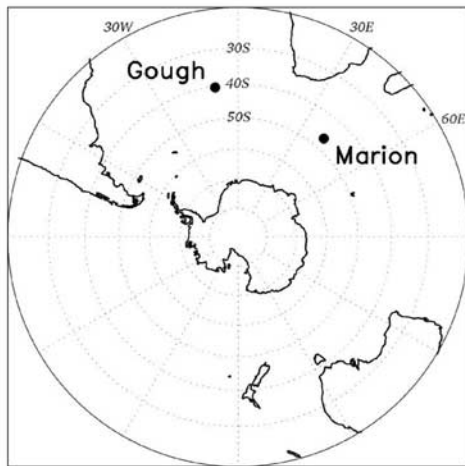
Figure 1. Locations of Gough ( 40^{\circ}20'S , 10^{\circ}0'W ) and Marion ( 46^{\circ}52'S , 37^{\circ}51'E ) islands.
