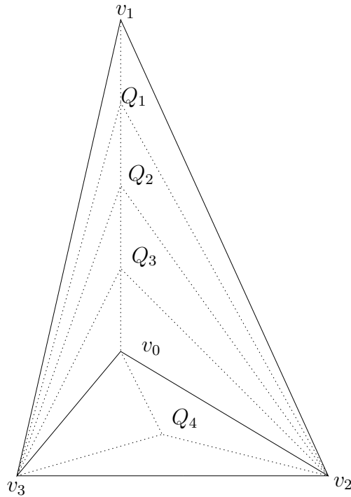
FIGURE 1. Polar polytopes of |\mathbb{P}(1, 3, 4, 4)| and crepant resolution
