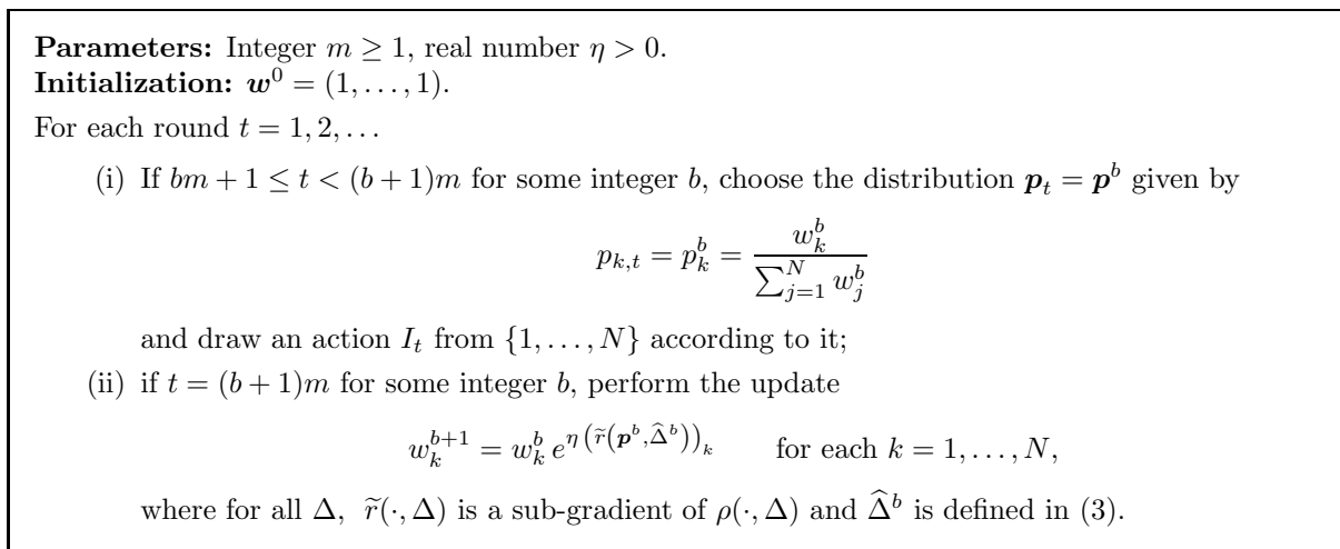
Figure 3: The forecaster for random feedback signals depending only on the outcome.
