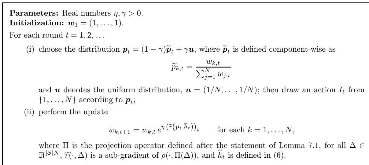
Figure 5: The forecaster for deterministic feedback depending on action–outcome pair.
