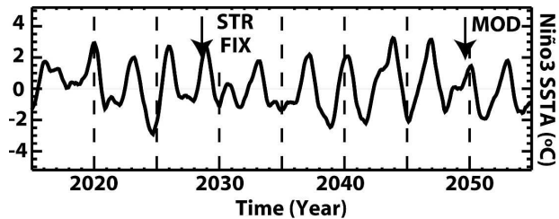
FIG. 1. Time series of interannual Niño-3 SST (°C) anomalies for the HadOPA coupled model from year 15 to 55. The anomalies are smoothed with a 5-month running mean. The arrows indicate the initial state of STR, FIX, and MOD ensembles.
