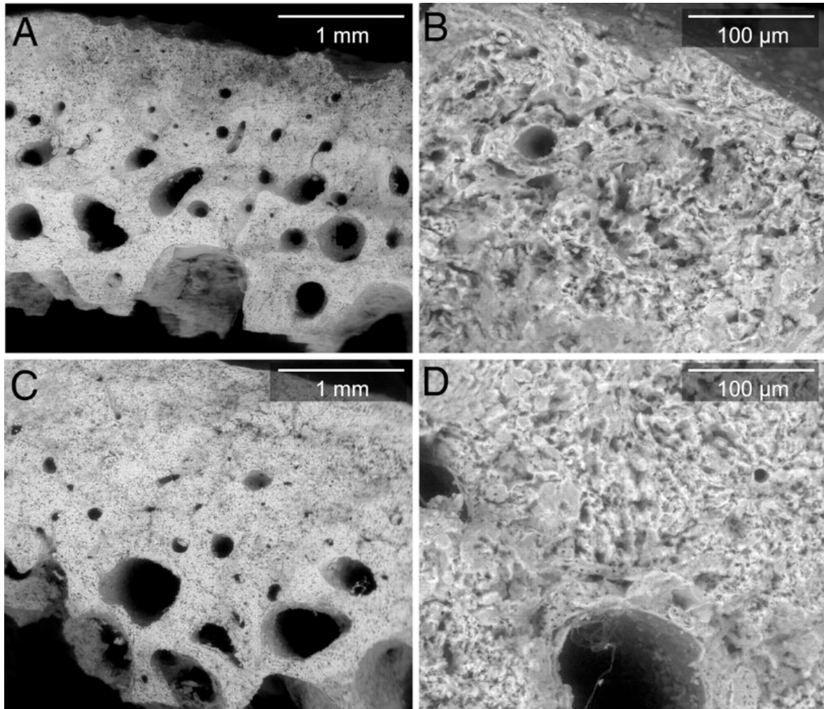
Fig. 2 Scanning electron microphotographs from cross-sections of two different fossil bone fragments from the aurochs ribs recovered from Pontvallain in 1947 (A and B) and in 2004 (C and D) (A and C, x40; B and D, x400)
