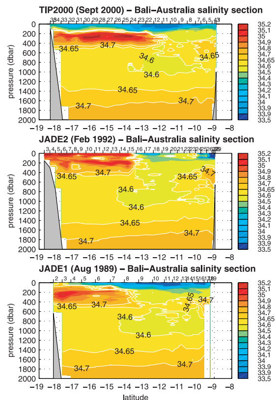
Figure 3. Salinity sections for JADE 1, JADE 2 and TIP cruises (the 34.65 isohaline denotes the NIIW).
