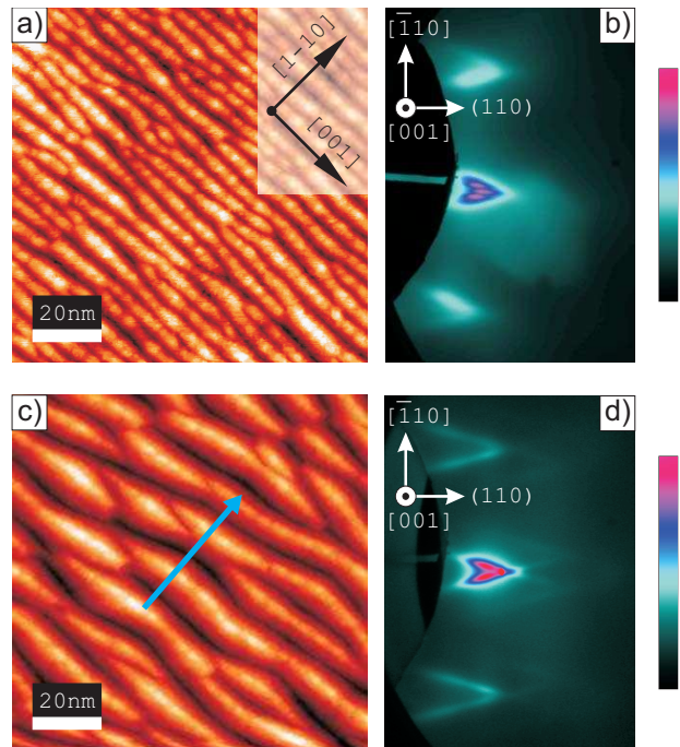
FIG. 1: W(110) templates: (a,c) 100 \times 100 \text{ nm} STM images of templates with small (a) and large (c) period, see text (b,d) RHEED patterns along the [001] azimuth for surfaces a and c, resp. The sample lies vertical, on the left of the patterns.
