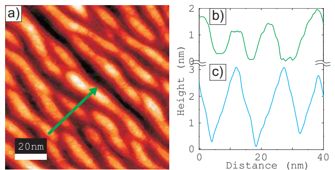
FIG. 2: (a) 100 \text{ nm} STM image of wires Fe(2.5 AL)/W (b) Cross-section along the line shown in (a) (c) Cross-section along the line shown in FIG. 1c (same scales).
