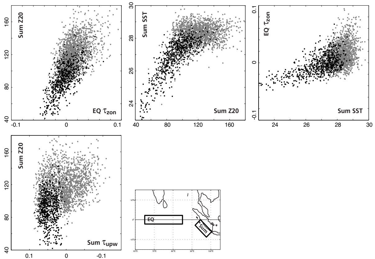
FIG. 12. Scatter plots of key absolute indices involved in the wind-thermocline-SST (Bjerknes-type) positive feedback from the noENSO simulation, with SON values in black, others in grey. From top, left to right, the zonal wind stress in an equatorial box spanning 60-90°E, 2°S-2°N vs. the 20°C isotherm depth in the box indicated off the coast of Sumatra, the Sumatra Z20 vs. Sumatra SST, and Sumatra SST vs. equatorial zonal wind stress. The lower left panel shows the relationship between the Sumatra alongshore upwelling component of the wind stress and Z20 in the same box.
