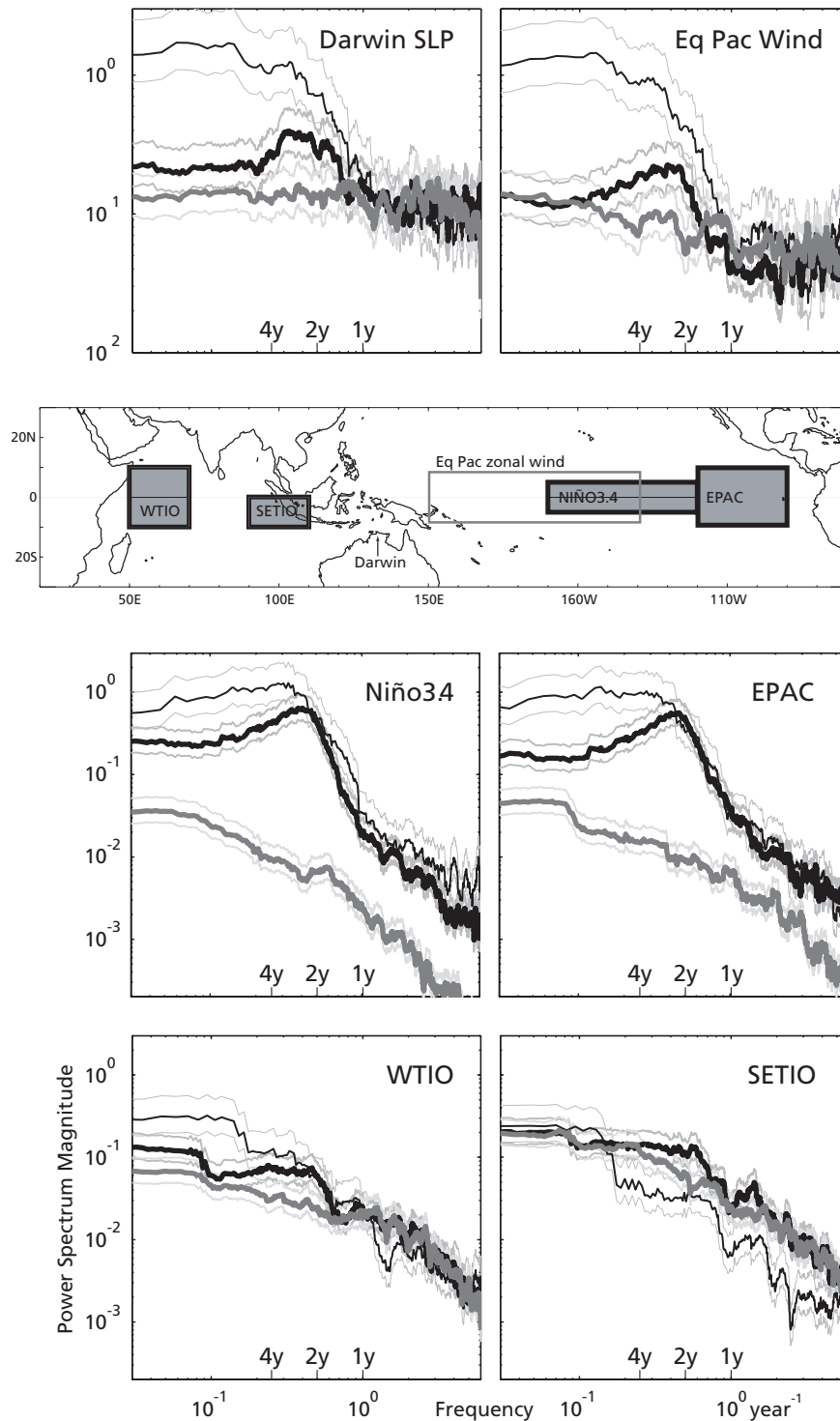
FIG. 5. Power spectra of representative atmospheric (Darwin, Australia sea level pressure and zonal wind in the equatorial Pacific, top 2 panels) and oceanic indices in the Pacific (the Niño3.4 and eastern equatorial Pacific SST anomaly indices, middle 2 panels) and Indian (WTIO and SETIO SST anomalies, bottom 2 panels) oceans, for climatological data (thin black line), and the REF (thick black line), and noENSO (thick grey line) simulations, calculated using the multi-taper method. Pale lines parallel to the main traces indicate the 95% confidence interval.
