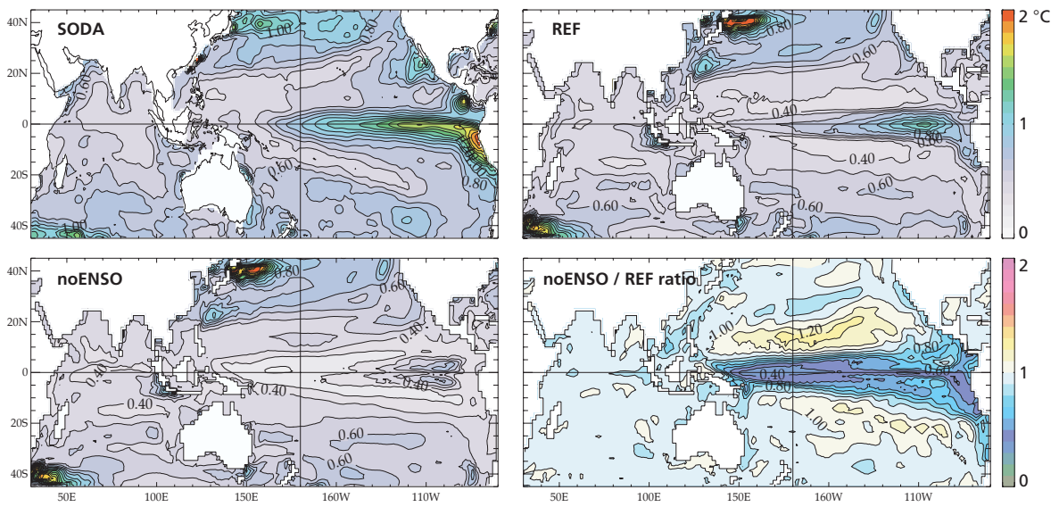
FIG. 3. Comparisons of the interannual variability in SST: standard deviation of the SST with respect to the mean seasonal cycle for the SODA analysis, and the runs REF and noENSO. The ratio of the standard deviations noENSO/REF is shown in the lower right panel.
