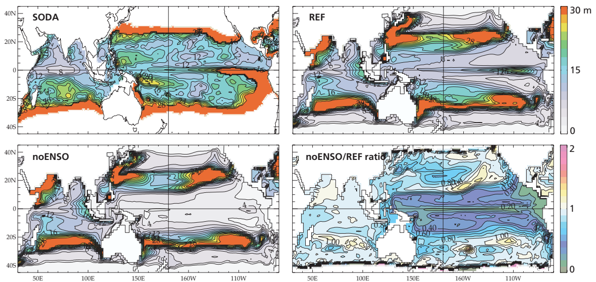
FIG. 4. Comparisons of the interannual variability in 20°C isotherm (Z20) depth: standard deviation of Z20 with respect to the mean seasonal cycle, for SODA data, the REF and noENSO simulations, and the ratio noENSO/REF.
