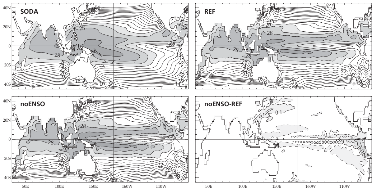
FIG. 1. Comparisons of mean SST for the SODA dataset, the 200-year reference run (REF), the 200-year wind-stress-constrained run (noENSO), and the difference between noENSO and REF. Mean panels have contour interval of 1°C and SST greater than 26°C is shaded grey. The difference panel has contour interval of 0.2°C, negative contours solid line, positive contour dashed line, with a maximum of 0.7°C just west of Peru at 12 °S.
