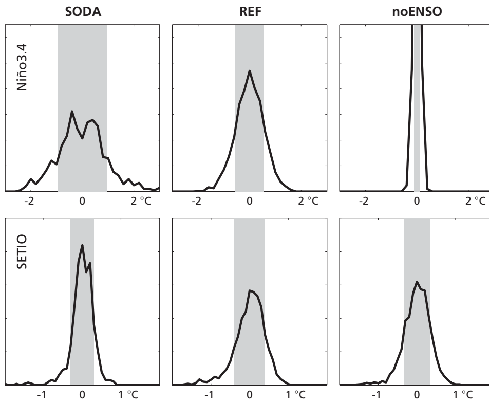
FIG. 9. Normalized histograms of the Niño3.4 and SETIO monthly SST anomaly timeseries from the SODA analysis, REF and noENSO. The vertical axis is arbitrary but to the same scale. The standard deviation of the distribution is marked by the grey shading. While Pacific variability has been effectively suppressed in noENSO, the SETIO remains nearly as active as REF. The negative tail in SETIO is somewhat reduced in the noENSO run, but still present.
