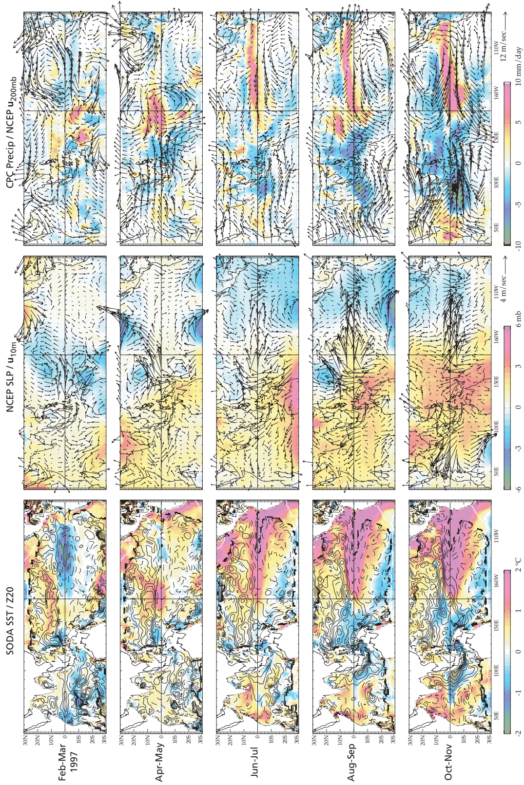
FIG. 19. As in Fig. 18, for 1997, a year with a concurrent IOZM event and strong El Niño.
