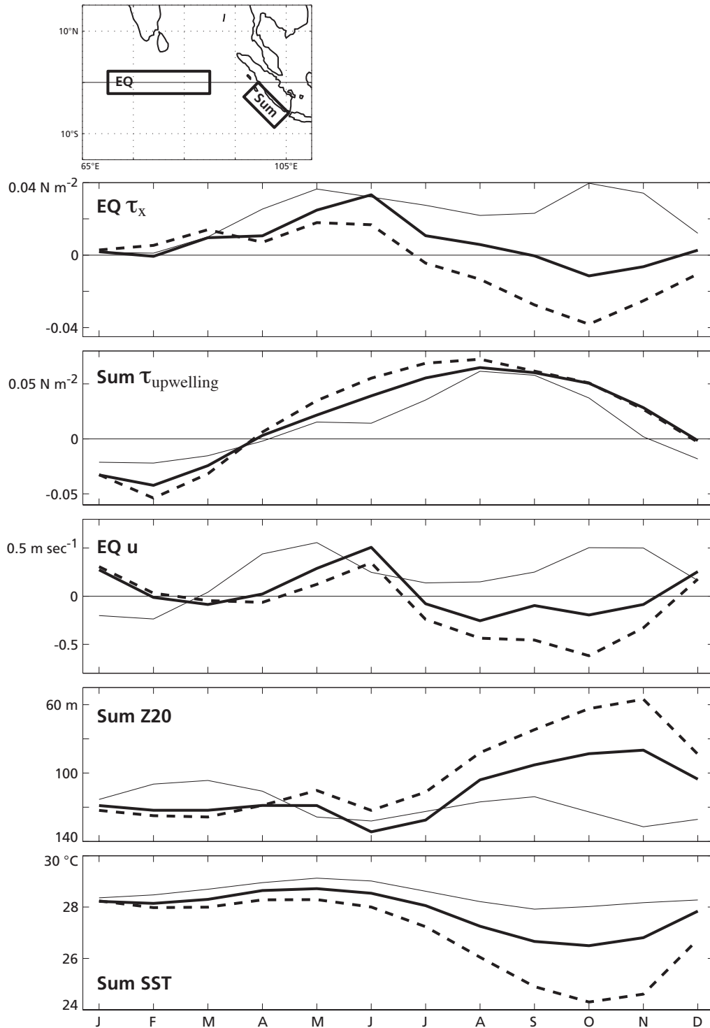
FIG. 2. The time evolution over one year of various indices important to the dynamical evolution of the IOZM, from: mean climatological observations (thin line), the mean seasonal cycle from the REF simulation (thick line), and the composite evolution during an IOZM event from the REF simulation (thick dotted line). For, from top: the zonal wind stress in an equatorial box ( 70\text{--}90^\circ\text{E} , 2^\circ\text{S}\text{--}2^\circ\text{N} ), the upwelling (exactly southeasterly) component of the wind stress in the box along the Sumatra coast (on map above, a rectangle 4^\circ wide and 8.5^\circ long oriented at an angle of 45^\circ to the equator), the zonal current in the equatorial box, the depth of the 20^\circ\text{C} isotherm, and SST, both in the Sumatra box. Climatological wind stress comes from SOC, oceanographic quantities from SODA. Quantities in the Sumatra box were averaged over oceanic grid points.
