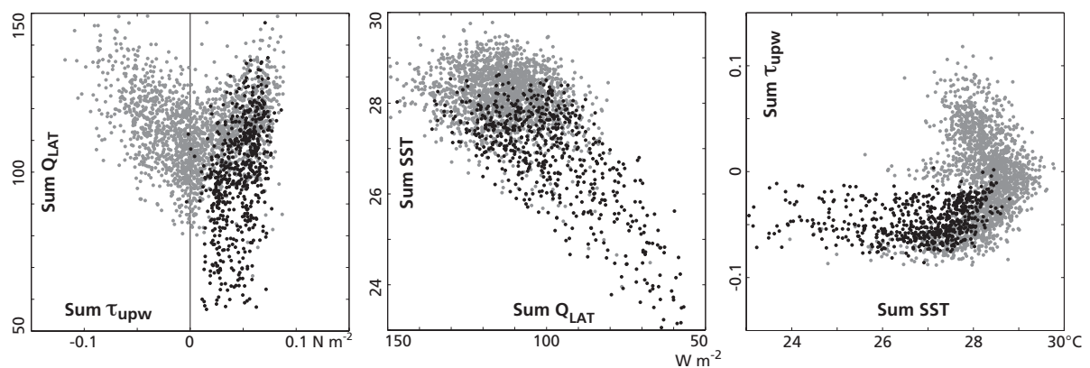
FIG. 13. Scatter plot of key indices involved in the wind-evaporation-SST coupled feedback from the noENSO simulation, SON values in black, others in grey. From left to right, the Sumatra alongshore component of the wind stress (which in all seasons is the major axis of the wind) vs. the Sumatra latent heat loss from the ocean, Sumatra latent heat loss vs. Sumatra SST, and Sumatra SST vs. Sumatra alongshore wind stress. This is not a positive feedback in the model during the IOZM season.
