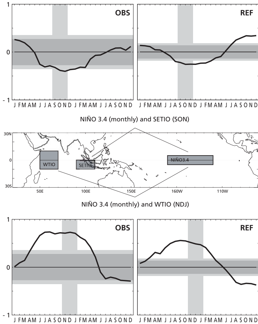
FIG. 6. Lead-lag correlations between seasonal indices of SST anomaly in the SETIO (top panels) and the WTIO (bottom panels) with the monthly Pacific Niño3.4 SST anomaly timeseries, in both observations (OBS, Reynolds and Smith, 1994) and the REF simulation. The dark and light horizontal bands delimit the 95 and 99% confidence intervals, while the season for the Indian Ocean index (SON for SETIO and NDJ for WTIO, the season of maximum interannual variability) is marked by the vertical band, showing the zero-lag correlation.
