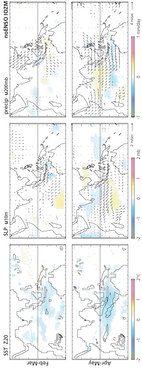
FIG. 14. Composite noENSO IOZM, triggering phase. This figure precedes Fig. 11 in time, with the same scaling and layout.
