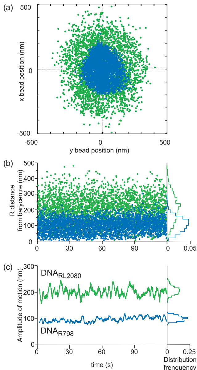
Figure 2. TPM calculation of the amplitude of motion. (a) Bead coordinates ( x, y ). Beads tethered to a glass support by DNA molecules, and therefore undergoing constrained Brownian motion, were tracked for 2 min (blue: \text{DNA}_{\text{R}798} ; green: \text{DNA}_{\text{RL}2080} ). (b) R positions as function of time. (c) Averaged amplitude of motion as a function of time.
