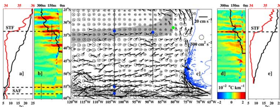
Figure 2. (a) SSS (red) and SST (black) along the 103^\circ\text{W} WOCE-P18 section; dashed lines correspond to the STF and the two SAF branch position. (b) meridional \theta gradient between 0–400 m depth along the P18 section (colour scale is given in Figure 2d); dashed lines show the front positions; thin black lines correspond to the 150 m and 300 m levels; thick black line corresponds to the 14^\circ\text{C} isotherms. (c) Surface velocities and velocity variance ellipses from drifter measurements; velocities higher than 6\text{ cm s}^{-1} are in bold; shaded areas indicate the STF (SSS in the range 34.3\text{--}34.8 ) and SAF positions (maximum \theta gradient in the range 3\text{--}8^\circ\text{C} at 100\text{--}400\text{ m} depth) identified from the WOA; observed STF and SAF positions are marked (blue dots) along both the WOCE-P18 and P19 sections (dotted lines); green dot corresponds to the STF identified from the study of Schneider et al. [2003]; (d) and (e): as (b) and (a) but along the 88^\circ\text{W} WOCE-P19 section.
