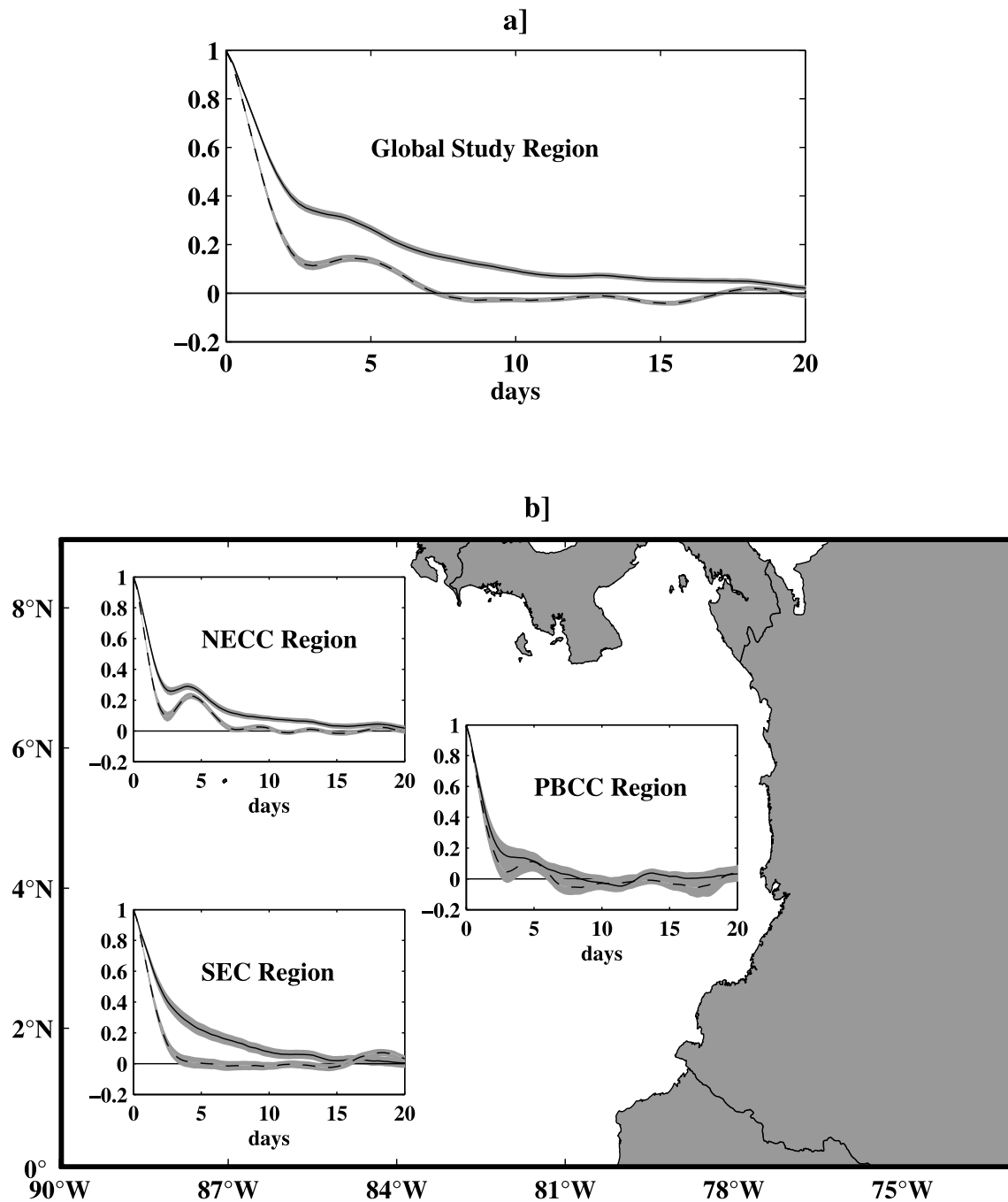
Figure 9. Temporal evolution of the normalized velocity autocorrelation functions. (a) whole study region and (b) NECC, PBCG and SEC regions. These were computed from zonal (solid lines) and meridional (dashed lines) velocity departures, relative to the seasonal circulation. The infrequent energetic events, as defined in the text, were previously removed.
