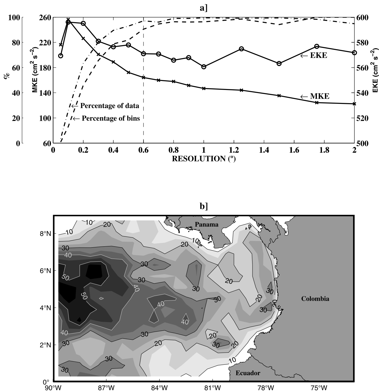
Figure 2. (a) Binned mean kinetic energy (MKE, crosses) and eddy kinetic energy (EKE, open circles), as a function of bin resolution. Also indicated are the percentage of considered bins (dashed line) and the percentage of data used in the estimates (dotted dashed line), as a ratio of data belonging to considered bins (see text) and the total number of data (65 656). Vertical dashed line corresponds to the spatial resolution of 0.6^\circ \times 0.6^\circ chosen to compute the near-surface characteristics of the mean flow. (b) Spatial distribution of independent observations per 0.6^\circ \times 0.6^\circ bins.
