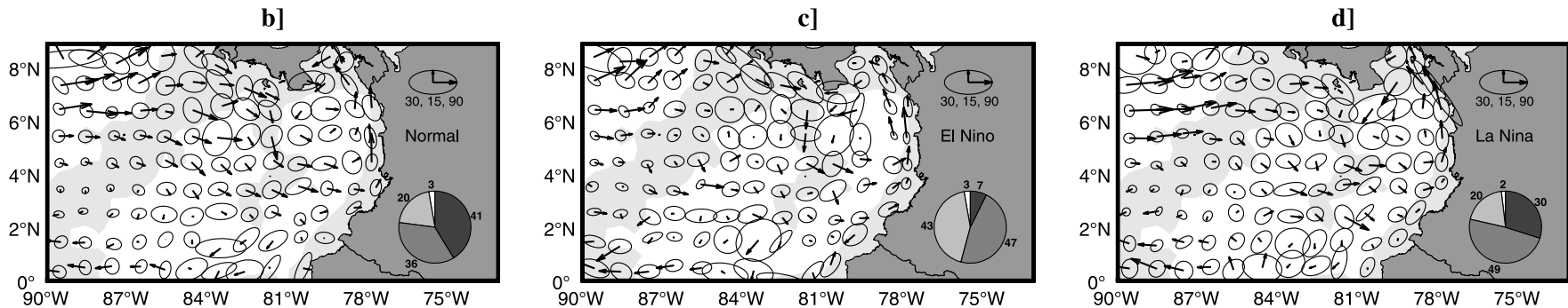
Figure 5. Distribution of the drifter data and mean circulation at interannual scales. (a) Niño3 Index computed from the monthly NCEP/NCAR sea surface temperature time series (see text) and monthly distribution of 6h drifter data between 1979 and 2004. Black (light grey, respectively) shade corresponds to El Niño (La Niña) periods whereas dark grey shade corresponds to “normal” conditions. (b)–(d) Surface circulation and velocity error ellipses computed from drifter data during “normal”, El Niño and La Niña periods. Arrows and ellipses are centered at the center of mass of the observations in each bin and the 0–2500 m depth range is shaded grey. Scale ellipses have a semimajor axis of 30 \text{ cm s}^{-1} , a semiminor axis of 15 \text{ cm s}^{-1} and are rotated 90^\circ from north. From white to black, pie parts indicate the percentage of bins having less than 3, 3 to 10, 10 to 20 and more than 20 independent observations, respectively.
