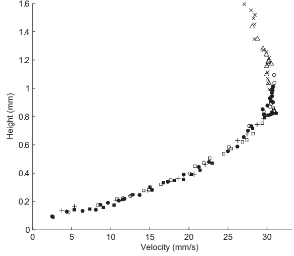
Fig. 3 Near-wall velocity profile of the density current, measured 0.3m downslope of the entrance with PST. Each symbol correspond to a different particle. \rho = 1025Kg.m^{-3} , Q = 0.95mL.s^{-1} , \theta = 16^\circ .
