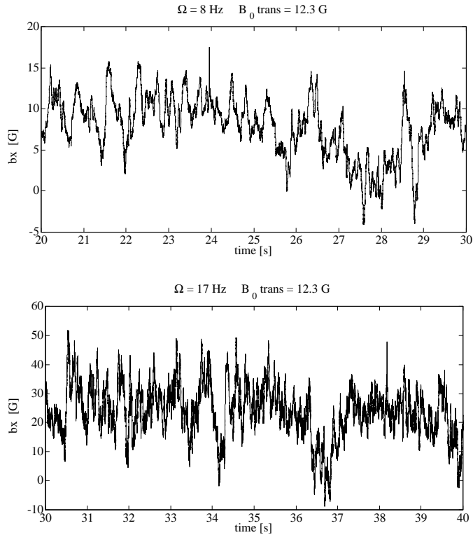
Figure 7. Time variation of the axial component of the induced field inside the flow, for a transverse applied field of magnitude B_0 = 12.3 G, at a rotation rate \Omega = 8 Hz (upper) and \Omega = 17 Hz (lower). The measurement probe is located near the mid-plane, 10 cm from the axis of rotation.
