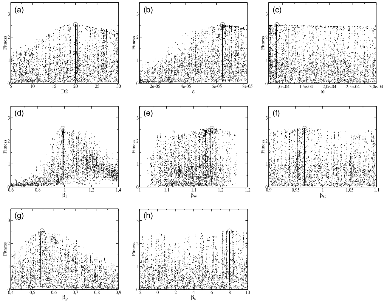
Figure 4. Fitness function obtained for each adjustable parameter: (a) D_2 ; (b) \epsilon ; (c) \omega ; (d) \beta_l ; (e) \beta_w ; (f) \beta_{st} ; (g) \beta_p ; and (h) \beta_s . The maximum fitness is circled.
