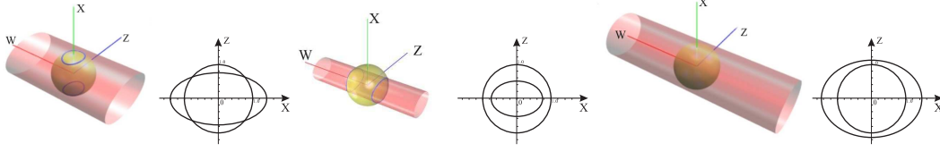
Fig. 2. Three cases of an elliptic cylinder intersecting with a unit sphere and their corresponding cross sections in the x - z plane.
