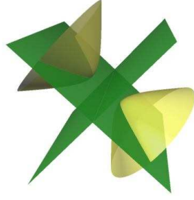
Fig. .5. The case of the QSIC having two conics, one real and one imaginary.
