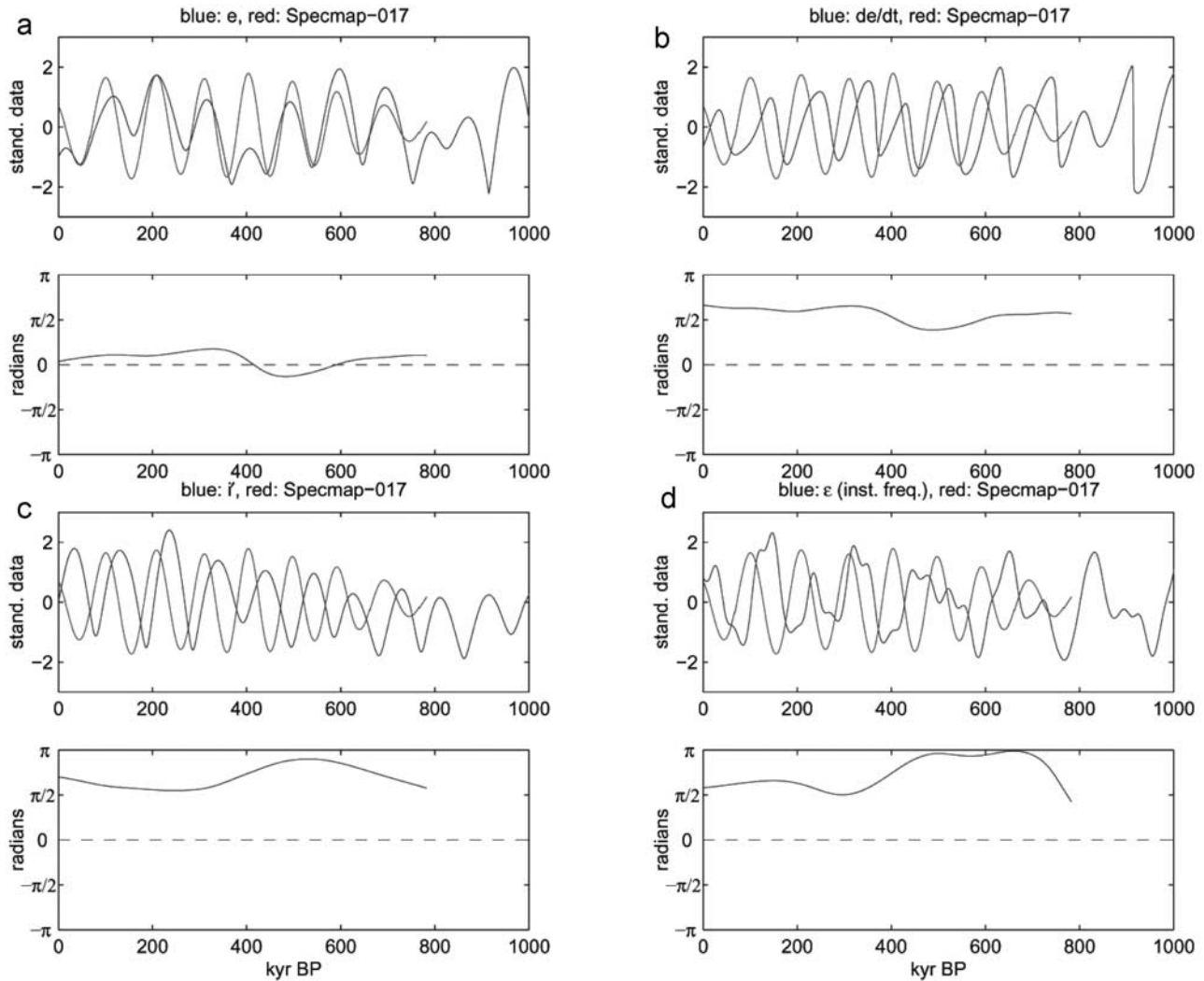
Figure 10. For the SPECMAP geological data shown in Figure 4, a cross-spectrum analysis is made with (a) e , (b) de/dt , (c) i , and (d) instantaneous frequency of \epsilon . In the top panel of Figures 10a–10d the extracted 100-kyr geological signal (red curve) is compared to the astronomical parameter (blue curve), and in the bottom panel the instantaneous phase difference is displayed. See color version of this figure at back of this issue.
