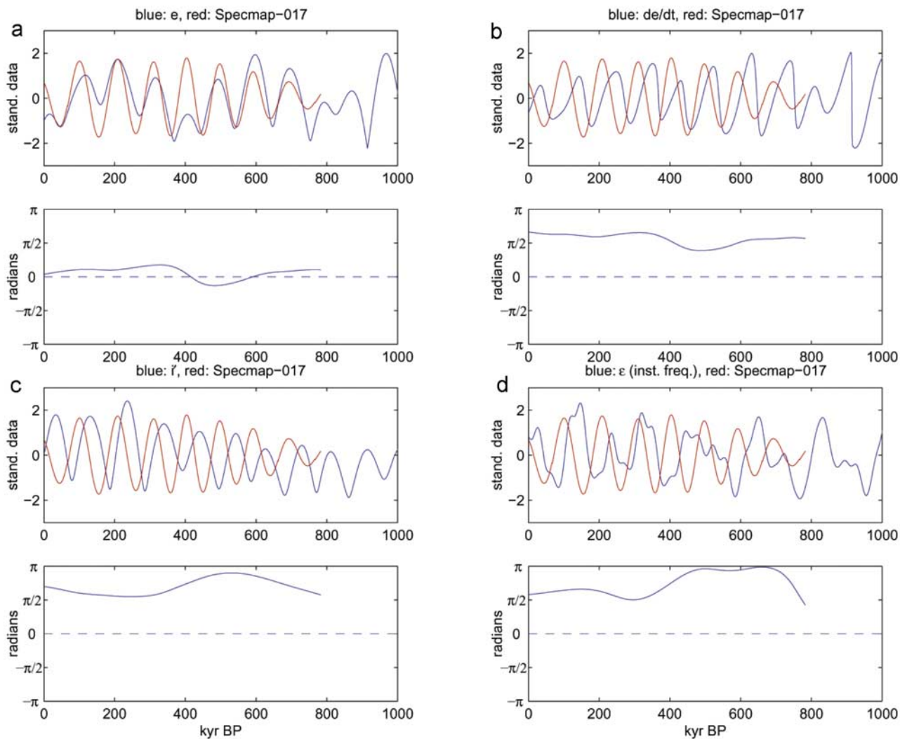
Figure 10. For the SPECMAP geological data shown in Figure 4, a cross-spectrum analysis is made with (a) e , (b) de/dt , (c) i' , and (d) instantaneous frequency of \varepsilon . In the top panel of Figures 10a–10d the extracted 100-kyr geological signal (red curve) is compared to the astronomical parameter (blue curve), and in the bottom panel the instantaneous phase difference is displayed.
