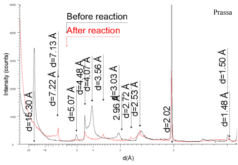
1005 Figure 7. X-Ray diffractograms of the Prassa-Fe(0) mixture before and after reaction at 80°C 1006 for 3 months, I/C=1/3.
