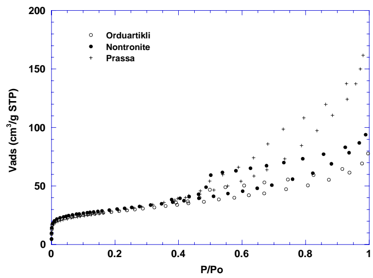
1009 Figure 8. Nitrogen adsorption/desorption isotherms at 77 K
