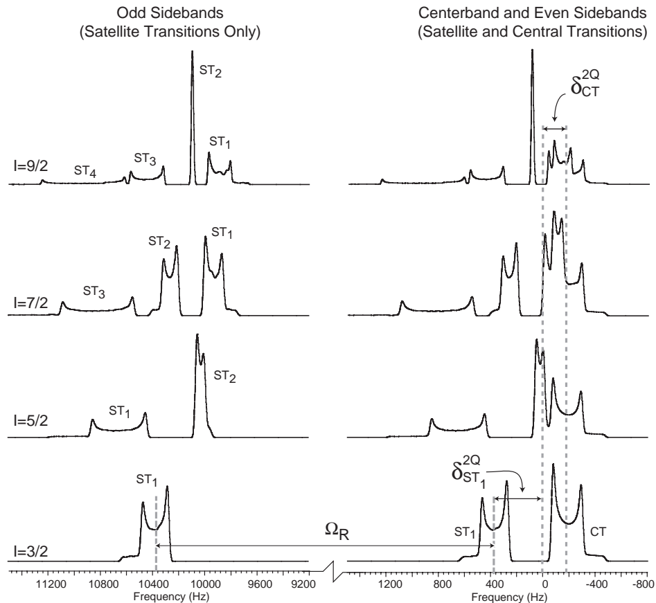
Fig. 3. Simulated central and satellite transitions spectra for spin I = 3/2, 5/2, 7/2, and 9/2 nuclei with C_q values of 1.0, 2.04, 3.13, and 4.24 MHz, respectively using half-rotor synchronized acquisitions to separate even and odd sidebands. The C_q value for each spin I was adjusted for constant central transition line widths ( \eta_q=0.0 and \nu_L=131.45 MHz). The second-order shifts[17] of the central ( \delta_{CT}^{2Q} ) and satellite transitions ( \delta_{ST}^{2Q} ) are given by \delta_{m,m-1}^{2Q} = \frac{-3[I(I+1) - 9m(m-1) - 3]}{40\nu_L^2 I^2 (2I-1)^2} C_q^2 \left(1 + \frac{\eta_q^2}{3}\right) \times 10^6 (ppm). For spin 7/2 and 9/2 nuclei, the central and the inner satellite transitions ( ST_1 ) overlap.
