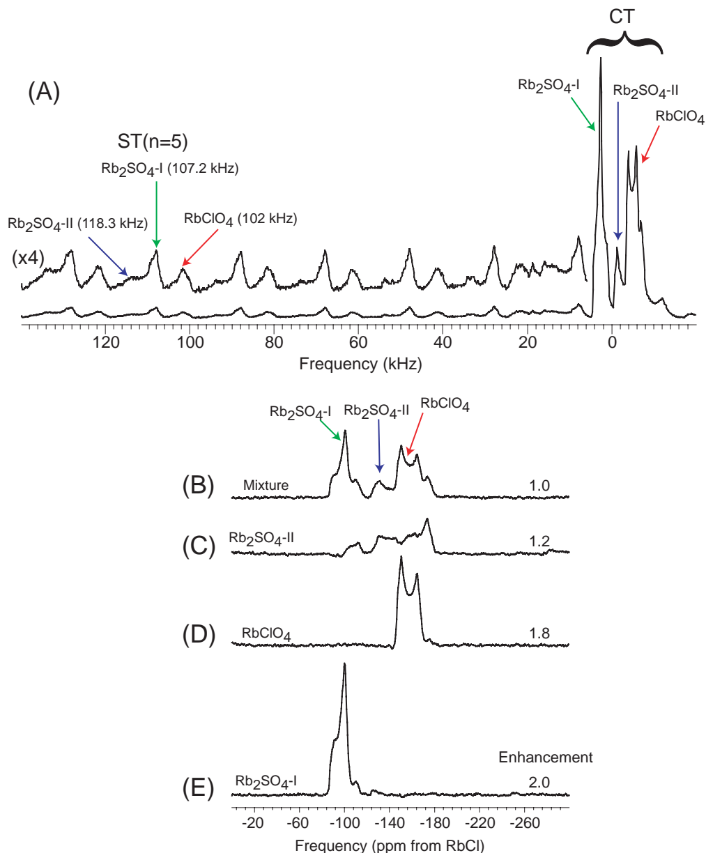
Fig. 4. (A) ^{87}\text{Rb} spectrum of a 1:1 mixture of polycrystalline \text{RbClO}_4 and \text{Rb}_2\text{SO}_4 [15,23] (40 k scans) acquired at a spinning rate of 20 kHz showing CT and ST signals. Only one side of the spinning sideband envelope is shown. (B) Single pulse spectrum (512 scans) (and (C)-(E) (\pi/2)_{\text{CT}}-(\pi)_{\text{ST}_1}-(\pi/2)_{\text{CT}} edited spectra (512 scans) for each site (CT region only). In each case, the inversion pulse was applied on one spinning sideband at the chosen offset as shown in (A). The adiabatic pulse parameters for the different sites are as follows: (C) \tau = 2 ms, excitation width = 8 kHz, \nu_{rf} = 8.5 kHz. (D) \tau = 5 ms, excitation width = 3 kHz, \nu_{rf} = 5.5 kHz. (E) \tau = 5 ms, excitation width = 3 kHz, \nu_{rf} = 5.5 kHz. The spectrometer offset was placed at the middle of the CT resonances to minimize the off-resonance effects that are caused by the low power read pulse.
