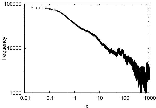
Figure 3: Figure 3. The correlation function at T=14 which shows a scaling region from about 0.3 to about 30, a range of about 2 decades with a scaling exponent \gamma = .42 .
