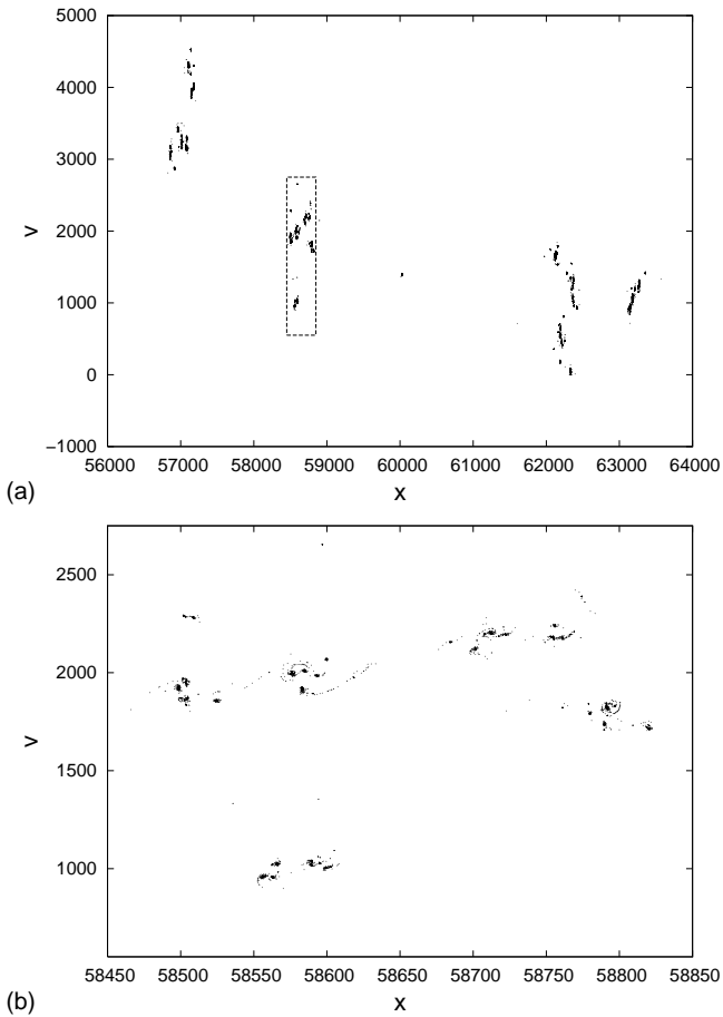
Figure 2: Consecutive expansions (zooms) on successive small squares selected in the \mu space panels at T=14 for the quintic model. They have the appearance of a random fractal which suggests self-similarity.
