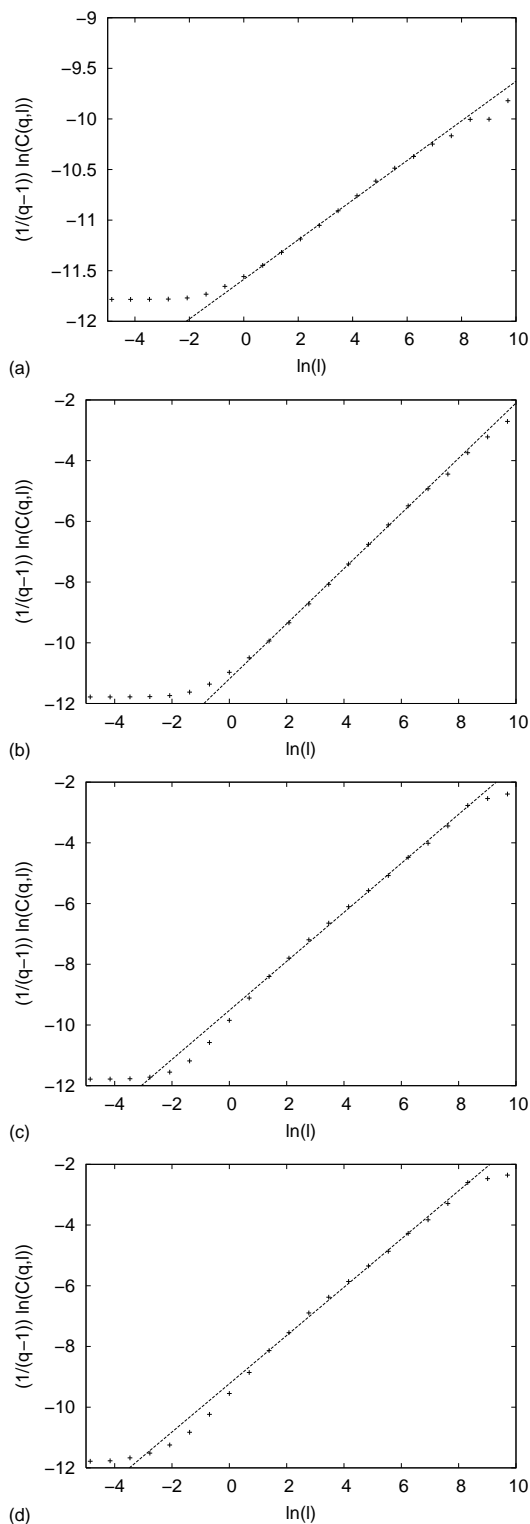
Figure 4: Scaling behavior in \mu -space. Plots of \frac{1}{q-1} \ln C_q versus \ln l are provided for four values of q : a) q=-5 , b) q=0 . c) q=5 , d) q=10 .
