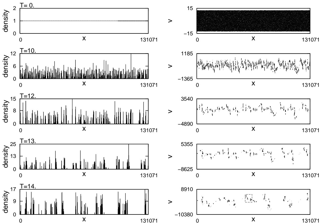
Figure 1: Evolution in configuration and \mu space for the quintic model with 2^{17} particles from T=0 to T=14 . The initial distribution is a waterbag with velocities in the range (-12.5, 12.5) and a size of about 16,000 Jeans' lengths.
