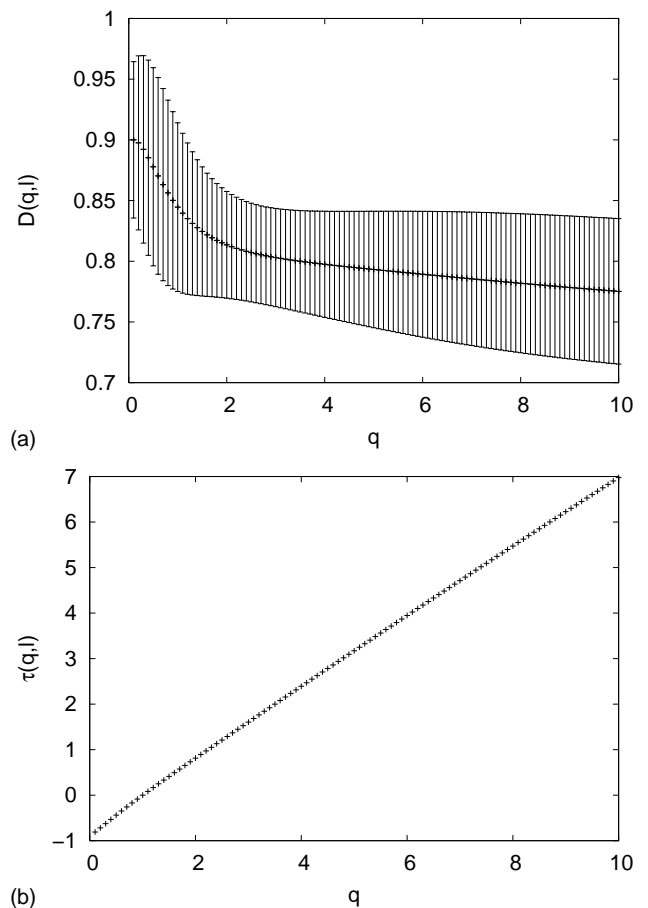
Figure 5: Generalized dimension D_q vs. q (panel a) and global scaling index \tau_q vs. q (panel b) in \mu -space for the quintic model at T=14 with q > 0 .
