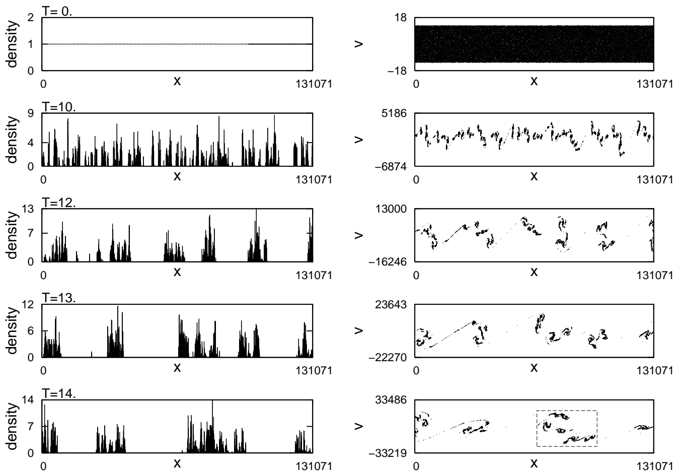
Figure 9: Evolution in configuration and space for the model without friction with 2^{17} particles from T=0 to T=14 . The initial distribution is a waterbag with velocities in the range (-14, 14) in the dimensionless units employed here and a size of about 10,400 Jeans' lengths.
