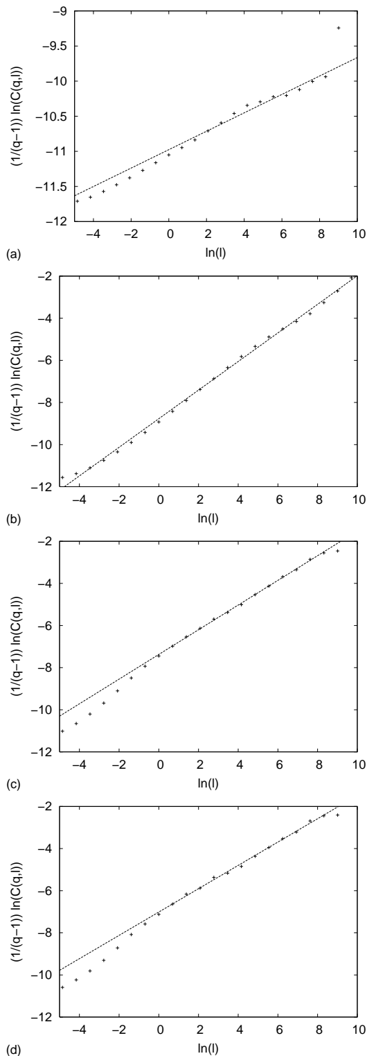
Figure 6: Plots of 1/(q-1)\ln(C_q) vs \ln(l) in configuration ( x ) space for the quintic model prepared as above at T=14 are provided for four values of q : a) q = -5 , b) q = 0 , c) q = 5 , d) q = 10 .
