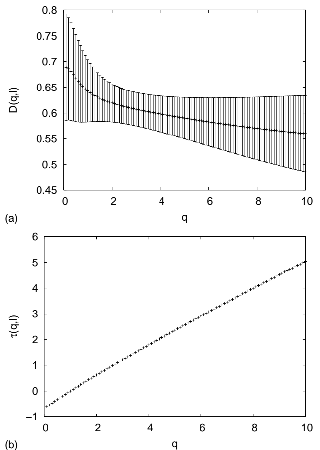
Figure 7: Generalized dimension D_q vs. q (panel a) and global scaling index \tau_q vs. q (panel b) in configuration ( x ) space for the quintic model at T=14 with q > 0 .
