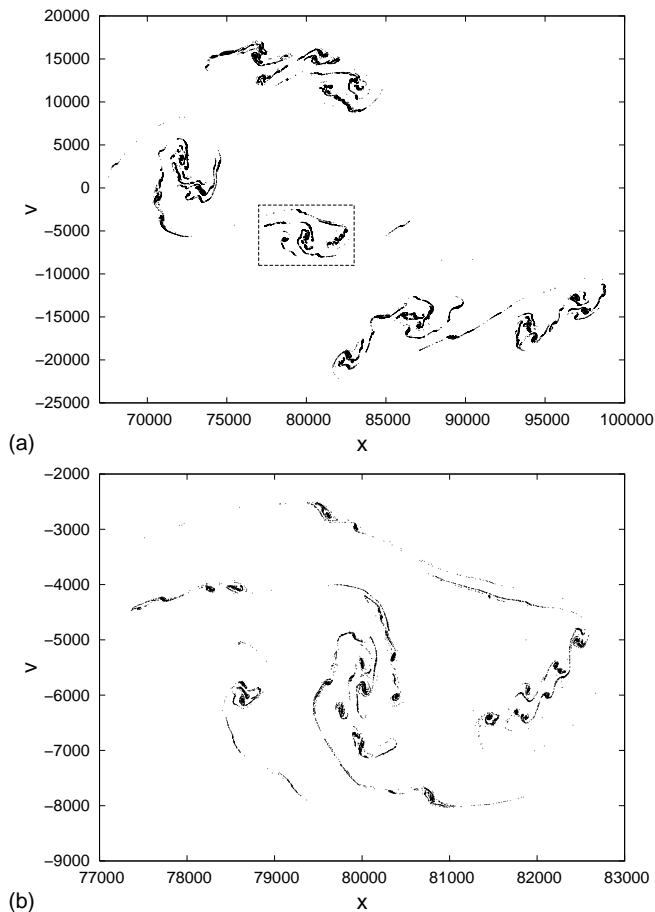
Figure 10: Consecutive expansions (zooms) of successive small squares (square within a square) selected in the \mu space panels at T=14 . They also have the appearance of a random fractal which suggests self-similarity.
