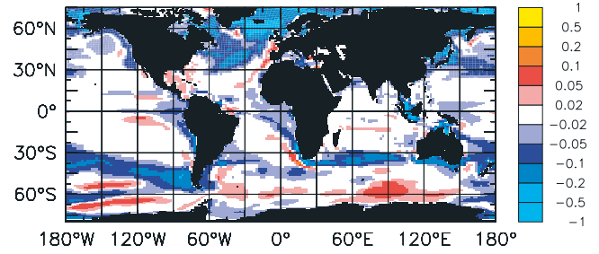
Figure 3. Simulated changes ( 4x\text{CO}_2 - 1x\text{CO}_2 ) in the relative abundance of diatoms.
