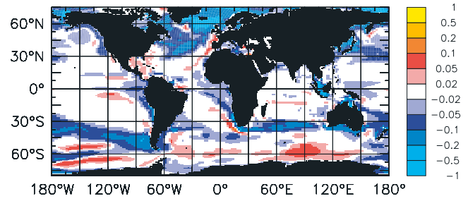
Figure 3. Simulated changes ( 4\text{xCO}_2 - 1\text{xCO}_2 ) in the relative abundance of diatoms.
