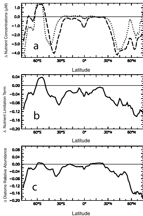
Figure 4. Zonal mean response to climate change ( 4\text{xCO}_2 - 1\text{xCO}_2 ) of (a) surface concentrations of nitrate (dashed line) and silicic acid (dotted line) in \mu\text{M} , (b) nutrient limitation term of diatoms growth, L_{lim} , see definition in the text, and (c) the relative abundance of diatoms.
