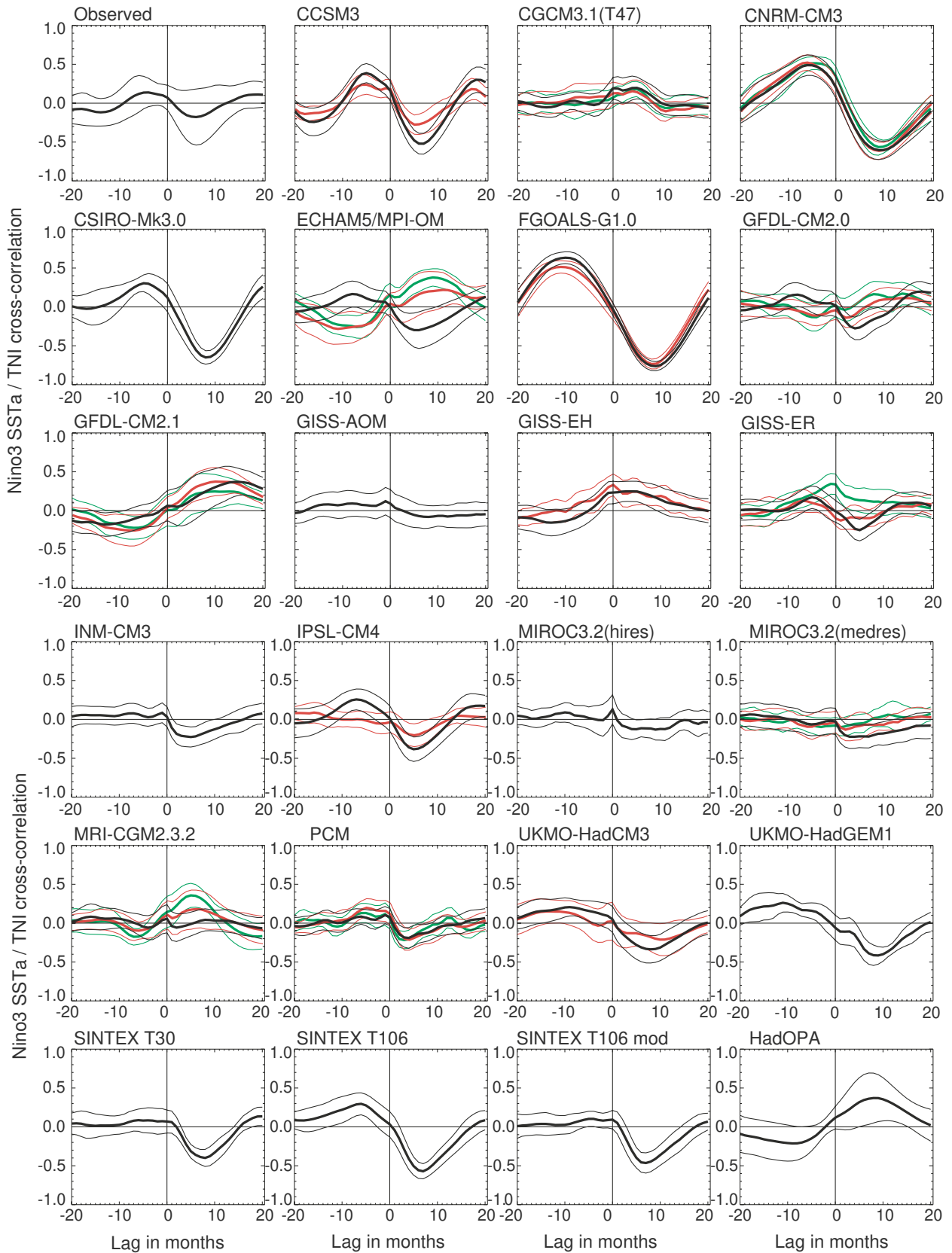
Fig. 12 The time mean lag-correlation of TNi and Niño3 SSTA ( thick line ), together with \pm 1 standard deviation ( thin lines ) for observations and all models and scenarios. Black picntrl, red 1pcto2x (after stabilization), green 1pcto4x (after stabilization)
