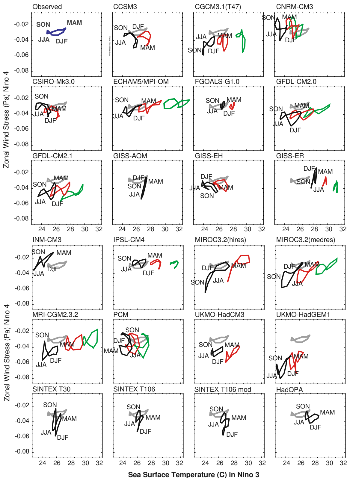
Fig. 4 Gill-like seasonal cycle for observations and for the models (after stabilization). Observed seasonal cycle is reproduced in grey as represent by Niño4 zonal wind stress ( \tau_x ) as a function of Niño3 SST. Black picntrl, red 1pctto2x (after stabilization), green 1pctto4x (after stabilization). Observed seasonal cycle is reproduced in grey for comparison. The position of the four seasons: MAM, JJA, SON, DJF is shown for the picntrl simulations
