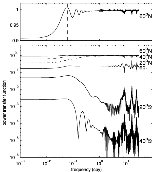
FIG. 3. Power transfer function for the meridional transport: D_T(y, \omega) = S_T(y, \omega)/S_{TN}(\omega) , at (top) 60^\circ\text{N} with linear axis, and (bottom) at several latitudes with logarithmic axis (the transports at 40^\circ and 20^\circ\text{N} are represented with dashed and mixed lines, respectively). The dashed vertical line (top) indicates the period of the gravest eigenmode.
