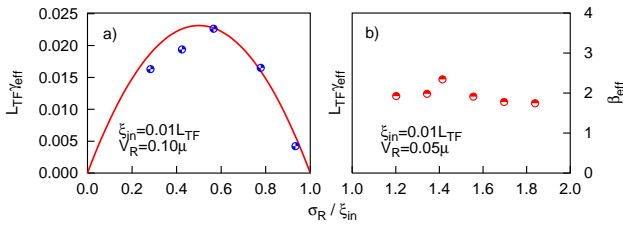
Figure 2: (color online) a) Lyapunov exponent \gamma_{\text{eff}} in units of 1/L_{\text{TF}} for the localized BEC in a speckle potential, in the regime \xi_{\text{in}} > \sigma_R . The solid line is \gamma(1/\xi_{\text{in}}) from Eq. (13). b) Exponent of the power-law decay of the localized BEC in the regime \xi_{\text{in}} < \sigma_R . The parameters are indicated in the figure.
