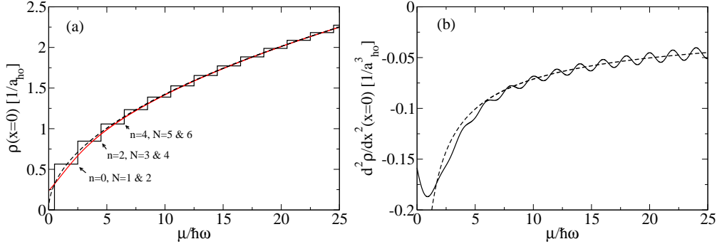
Fig. 3. – (Color online) Central density of a 1D harmonically trapped ideal Fermi gas, in the grand canonical ensemble, as a function of the chemical potential \mu . (a) Density in the trap center x = 0 : exact result for T = 0 (black solid line), exact numerical sum for k_B T = \hbar\omega (red solid line), vs the T = 0 LDA (dashed line). (b) Second order derivative of the density in the trap center, d^2\rho/dx^2(x=0) , for k_B T = \hbar\omega : exact numerical sum (solid line) vs the T = 0 LDA (dashed line).
