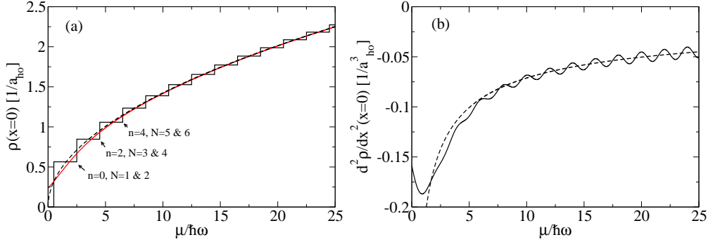
Fig. 3. – (Color online) Central density of a 1D harmonically trapped ideal Fermi gas, in the grand canonical ensemble, as a function of the chemical potential \mu . (a) Density in the trap center x = 0 : exact result for T = 0 (black solid line), exact numerical sum for k_B T = \hbar\omega (red solid line), vs the T = 0 LDA (dashed line). (b) Second order derivative of the density in the trap center, d^2\rho/dx^2(x=0) , for k_B T = \hbar\omega : exact numerical sum (solid line) vs the T = 0 LDA (dashed line).
