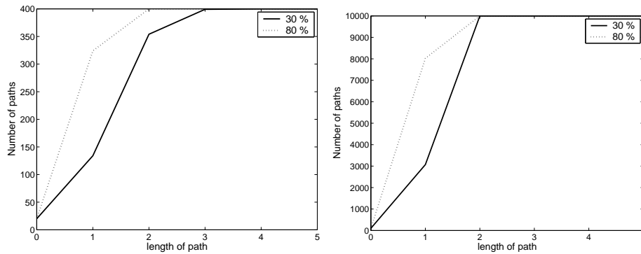
Fig. 2. Number of paths of a given length simulation in a random graph. (left) Graph order is 30. (right) Graph order is 100. The two curves in each plot depends on the percentage of graph connectivity.
