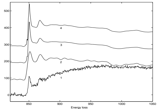
Fig. 2: An example of EELS deconvolution. To improve the readability of the figure the different curves are shifted with a constant value. Curve 1 corresponds to the EELS spectrum, curve 2 to the deconvoluted spectrum obtained by the Egerton method. Curves 3 and 4 correspond to the deconvoluted spectrum obtained by the proposed approach for different values of the regularization parameter \lambda .
