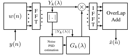
Fig. 1: Block diagram of a single channel signal denoising algorithm.
