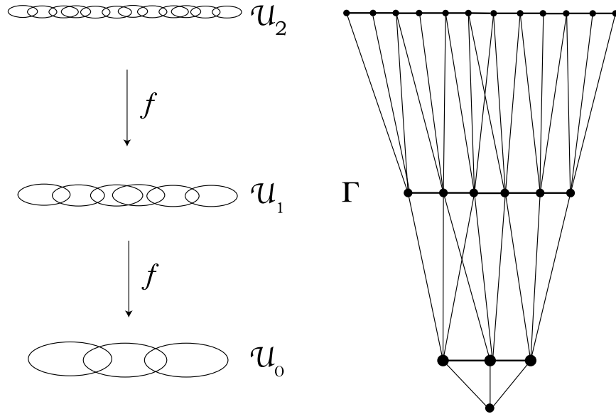
Figure 3.2: Definition of the graph \Gamma .
