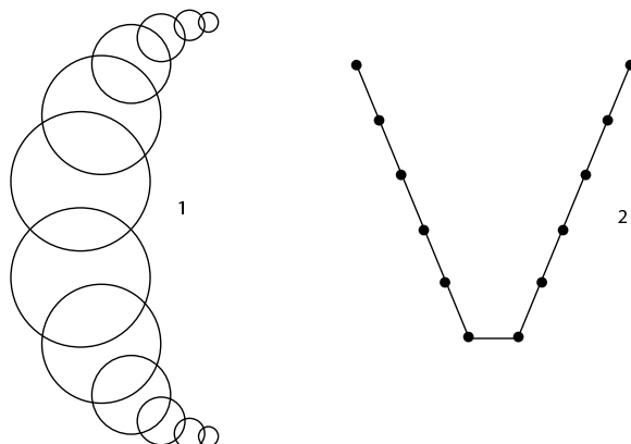
Figure 3.3: The vertices of a parameterized edge-path in \Gamma , at right, correspond to a sequence of elements of \mathbf{U} in which consecutive elements intersect in points of the repellor, X .
