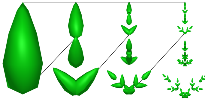
Fig. 2. Construction of an artificial crown. The initial object was a tapered ellipsoid and the IFS transformation was made of n = 5 duplications of a contracted object by a factor c = 3 .
