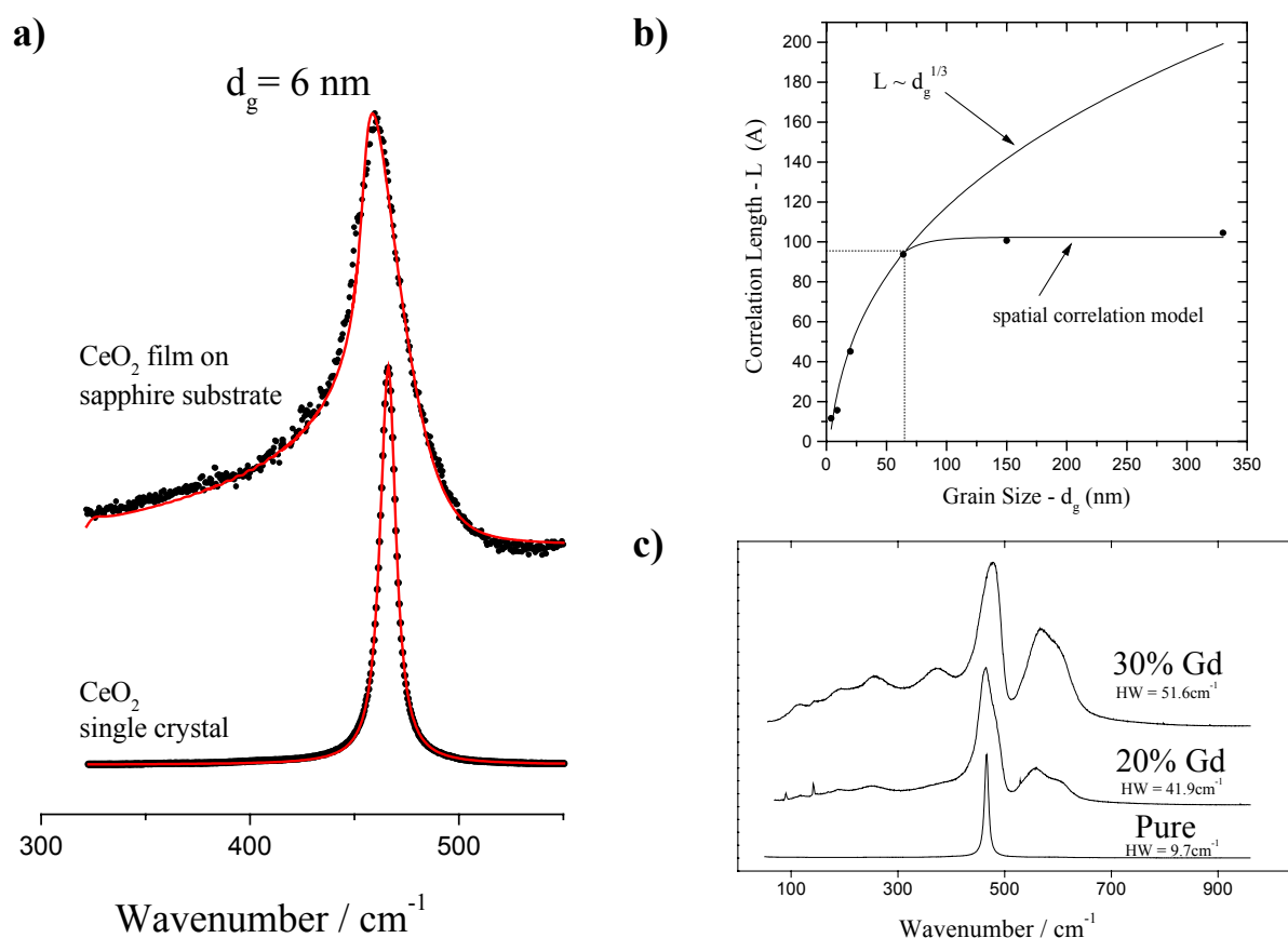
Figure 18 : a) Grain size effect on ceria Raman signature. The fits were obtained using the PCM (§ 3.3.1) – b) Comparison of the confinement length L obtained through the PCM with the grain size obtained by X-ray diffraction. Reprinted from Solid State Ionics, 149[1-2], I. Kosacki et al. , Raman scattering and lattice defects in nanocrystalline \text{CeO}_2 thin films, pp 99-105, 2002, with permission from Elsevier – c) The spectra of gadolinium-doped ceria single crystals highly depend on the doping level (I. Kosacki and Ph. Colomban, Private Communication)
