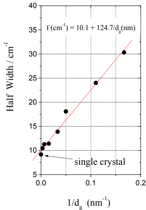
Figure 6 : The half-width at half height of \text{CeO}_2 Raman band ( 466 \text{ cm}^{-1} ) plotted as the inverse of the grain size obtained by X-ray diffraction. Reprinted from Solid State Ionics, 149[1-2], I. Kosacki et al. , Raman scattering and lattice defects in nanocrystalline \text{CeO}_2 thin films, pp 99-105, 2002, with permission from Elsevier.
