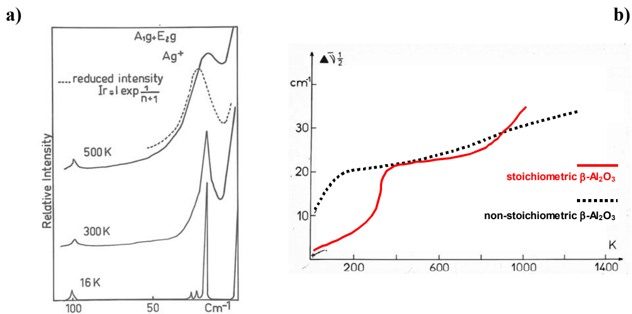
Figure 13 (Adapted from Ph. Colomban et al. , J. Chem. Phys., 75[3], pp 1388-1399, 1981) a) The \sim 25 \text{ cm}^{-1} peak of \beta -alumina is characteristic of the conducting short range ordered \text{Ag}^+ bi-dimensional sub-lattice - b) The half-width of the peak makes it possible to identify the melting temperature of the sub-lattice.
