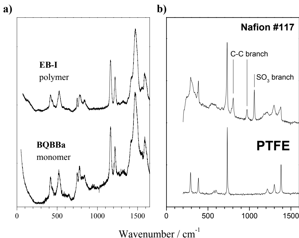
Figure 12 : a) Comparison between the spectra from polyaniline precursor monomer (1 ~1 nm) and polyaniline in one emeraldine base form ( 1 ~ 200 nm) (Adapted from S. Folch et al. , Macromol., 32, 3080, 1999) – b) Comparison of PTFE and Nafion (PTFE-grafted with sulfonic groups) Raman spectra (Adapted from A. Gruger et al. , Vibr. Spectr., 26, 215, 2001).
