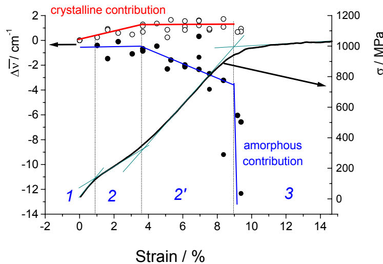
Figure 27 : Comparison of the strain dependency of the crystalline and amorphous low frequency Raman contributions (left hand scale) with the stress-strain tensile curve (right hand scale) for PET fibres. Reprinted from Engineering Fracture Mechanics, 73[16], Ph. Colombari et al. , Micro-Raman study of the fatigue and fracture behaviour of single PA66 fibres: Comparison with single PET and PP fibres, pp 2463-2475, 2006, with permission from Elsevier.
