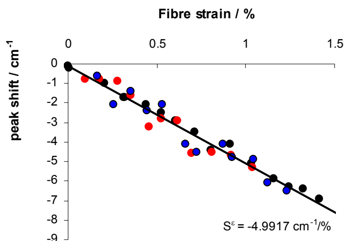
Figure 20 : Calibration of the Raman Mechanical Coefficient ( S^{\varepsilon/\sigma} ) of carbon G band (see § 4.3) for 3 IM7 fibres (Adapted from Ph. Colomban et al. , Composites Part A, 37[4], pp 646-651, 2006).
