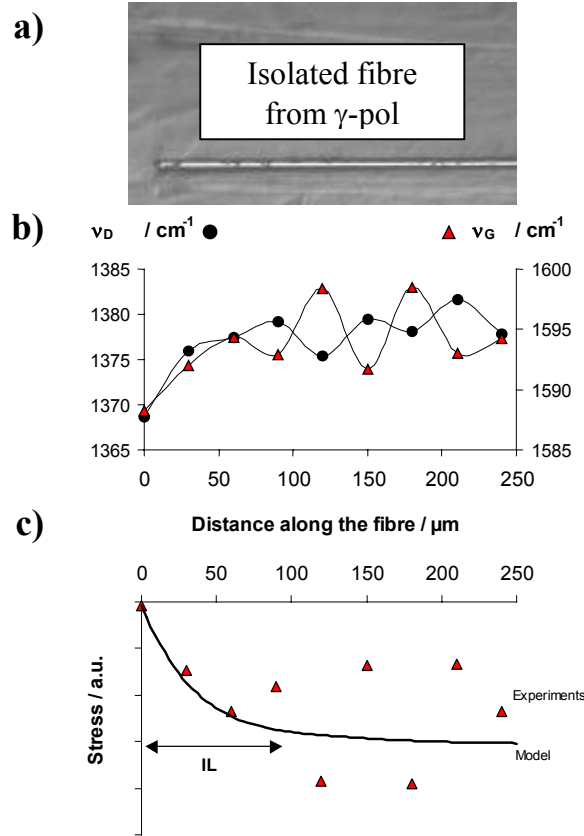
Figure 23 –Raman stress measurement in opaque industrial \text{C}_f /epoxy composites submitted to tensile strain, Reprinted from Composites Part A, 37[4], Ph. Colomban et al. , pp 646-651, 2006, with permission from Elsevier - a) Optical micrograph of an IM7 fibre entering the matrix of " \gamma -pol" composite (see text) strained to 1% - b) Wavenumber variations along the same fibre (origin at fibre tip, \lambda_{\text{laser}}=457.9\text{nm} , P_{\text{illumination}}=1.5\text{ mW} ) - c) modelling of \nu_G -derived axial compressive stress along the same fibre (IL: Ineffective Length) [486].
