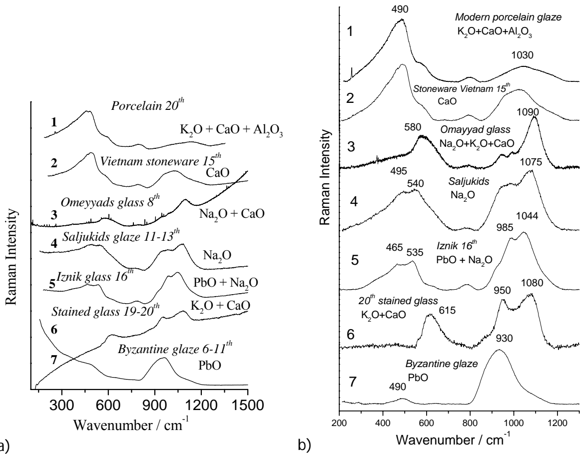
Fig. 4 : Representative Raman spectra for the 7 families identified : a) as-recorded spectra; b) baselines have been subtracted in order to only keep the "SiO 4 " molecular signature (the contribution of the "Boson peak" is eliminated).
