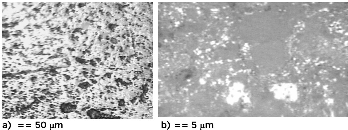
Figure 5: Typical optical micrographs of red polished stoneware body (a, b, MNC308), ewer stopper body (b) and glaze (b', MNC2274). Note the of the large quartz grain, with concave interface indicating a dissolution by a very active liquid flux.
