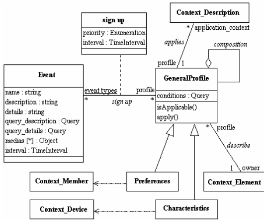
Figure 4. UML schema describing the General Profiles.
