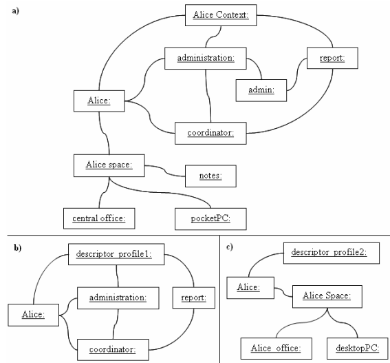
Figure 6. Graphs generated by the context description instances associated to Alice's current context (a) and her profiles (b) (c) .
