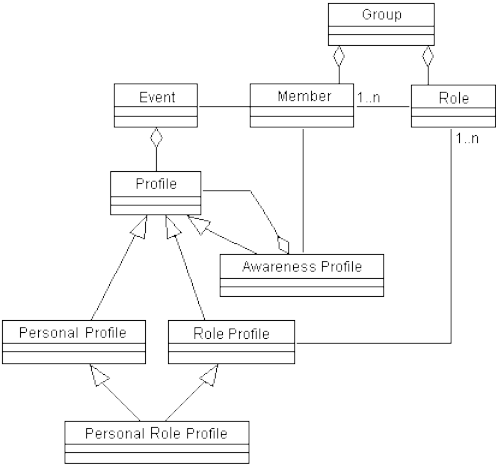
Figure 4. Some Kernel package internal classes
