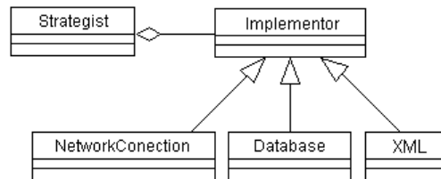
Figure 5: Storage package details
