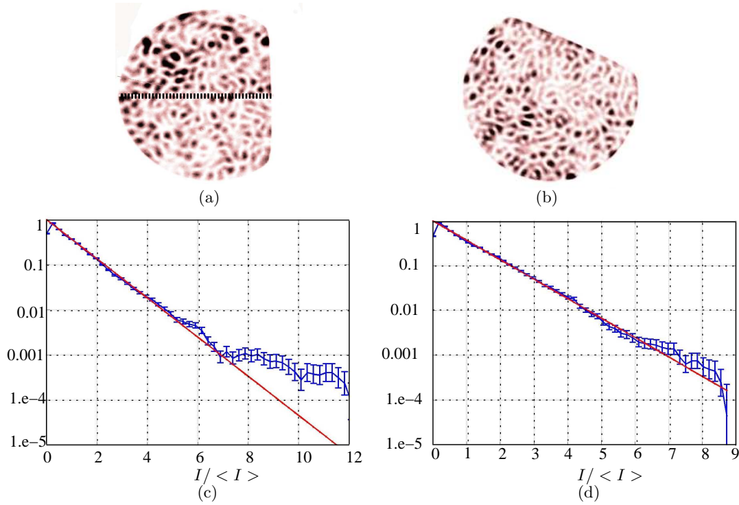
Fig. 7. NF intensities and their respective probability distribution for an input illumination along the 2-bounce PO (a), (c) and for the rotated fiber (b), (d).
