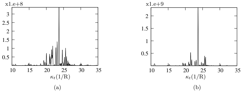
Fig. 12. Evolution of the intensity spectrum along the propagation (a) at z=0cm , (b) z=80cm .
