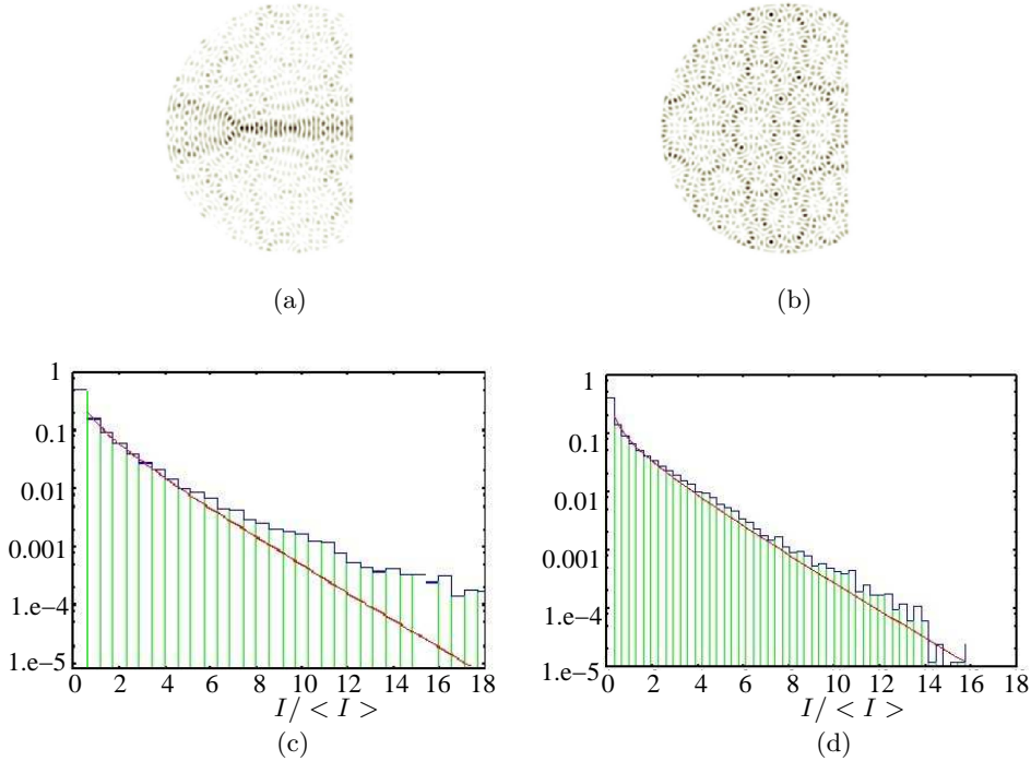
Fig. 6. Intensity of the field associated to calculated scar mode (a) and speckle mode (b) and their respective probability distribution of intensity (c) and (d).
