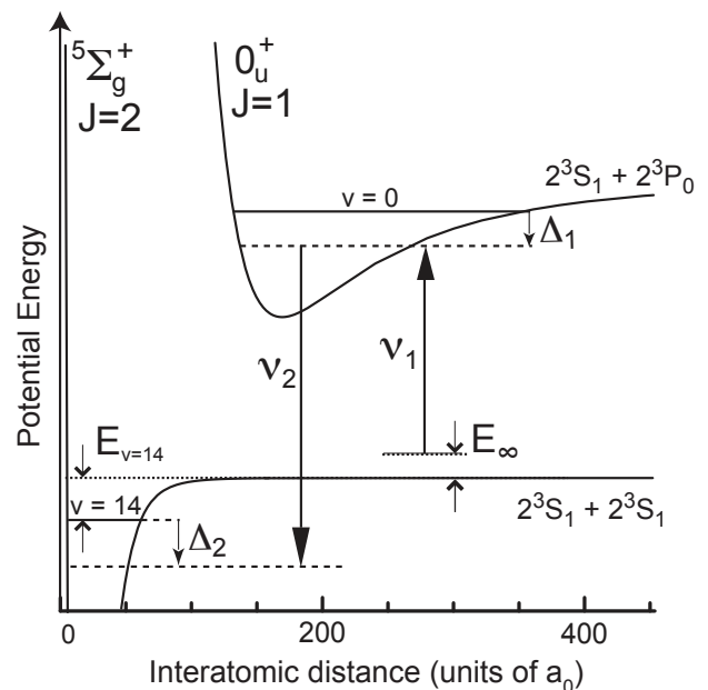
FIG. 1: Levels involved in the two-photon photoassociation experiment. {}^5\Sigma_g^+ is the interaction potential between two spin-polarized 2^3S_1 helium atoms, v = 14 being the least-bound vibrational state in this potential. Laser L_1 at frequency \nu_1 operates on the free-bound transition with a detuning \Delta_1 , and laser L_2 at frequency \nu_2 drives the bound-bound transition with a detuning \Delta_2 from the two-photon transition. Energies are not to scale.
