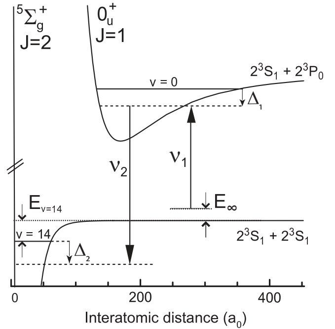
FIG. 1: Levels involved in the two-photon photoassociation experiment. {}^5\Sigma_g^+ is the interaction potential between two spin-polarized 2^3S_1 helium atoms, v = 14 being the least-bound vibrational state in this potential. Laser L_1 at frequency \nu_1 operates on the free-bound transition with a detuning \Delta_1 , and laser L_2 at frequency \nu_2 drives the bound-bound transition with a detuning \Delta_2 from the two-photon transition.
