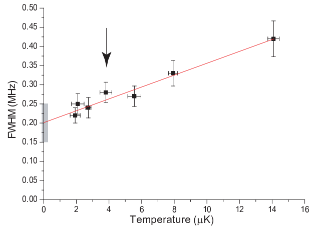
FIG. 9: FWHM of the Raman peak versus temperature of the atomic cloud. The temperature is changed by adjusting the evaporative cooling stage. The experimental parameters are fixed to I_1 = 660 \text{ mW/cm}^2 , I_2 = 66 \text{ mW/cm}^2 , \tau_{PA} = 200 \text{ } \mu\text{s} , \Delta_1 - \Delta_2 = 20 \text{ MHz} .
