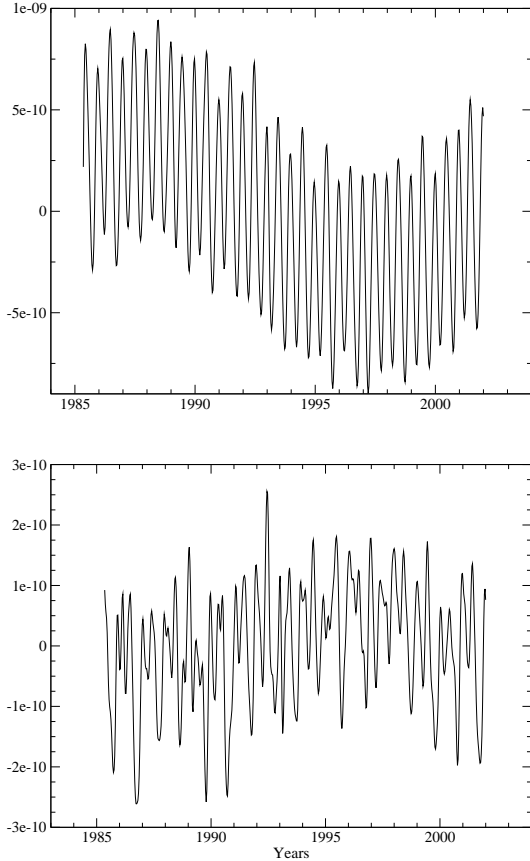
Fig. 7. Normalized total \Delta C_{20} : top is the total series including atmospheric, oceanic tides and solid earth tides effects and the residuals; bottom is the total series without the solid earth tides effect.
