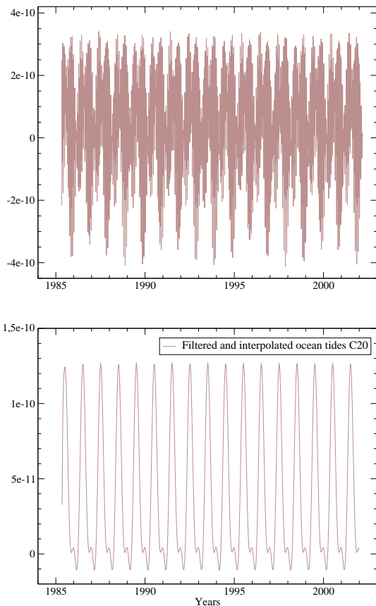
Fig. 5. Normalized oceanic \Delta C_{20} (top: raw data, bottom: filtered data, where the high frequency signals have been removed): oceanic-tide-modelled part of the \Delta C_{20} harmonic coefficient of the Earth gravity field; IERS Conventions 1996.
