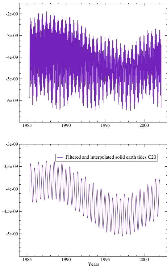
Fig. 6. Normalized solid tides \Delta C_{20} (top: raw data, bottom: filtered data, where the high frequency signals have been removed): solid-Earth-tide-modelled part of the \Delta C_{20} harmonic coefficient of the Earth gravity field; IERS Conventions 1996.
