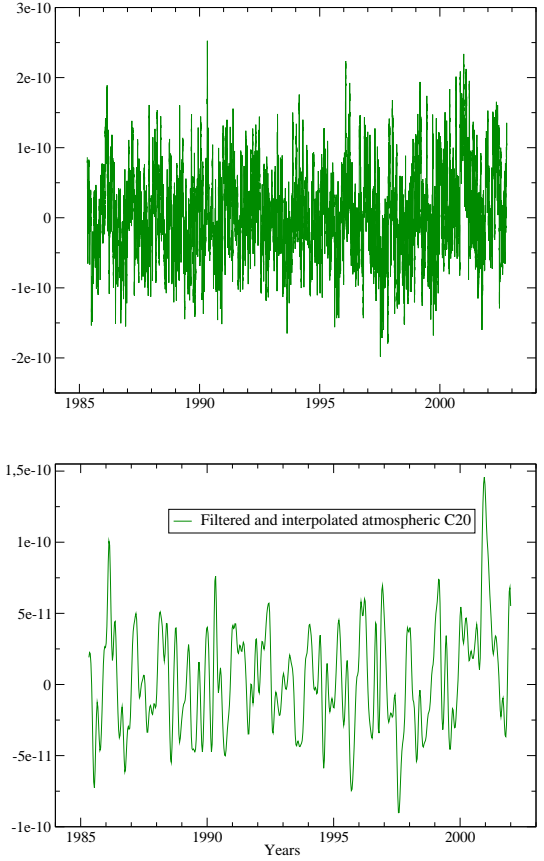
Fig. 4. Normalized atmospheric \Delta C_{20} (top: raw data, bottom: filtered data, where the high frequency signals have been removed): atmospheric modelled part of the \Delta C_{20} harmonic coefficient of the Earth gravity field, obtained with ECMWF pressure data.
