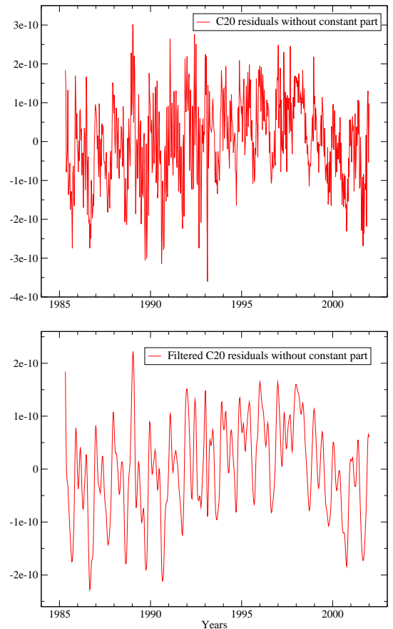
Fig. 2. Normalized \Delta C_{20} residuals (top: raw residuals, bottom: filtered residuals, where the high frequency signals have been removed): non-modelled part of the \Delta C_{20} harmonic coefficient of the Earth gravity field.
