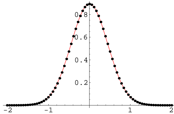
Figure 6: Discrete probability mass function \sigma_{256} f_{256}(x\sigma_{256}) (discrete points) and y = \sigma_{256} f_{256}(0)e^{-\pi f_{256}(0)^2 \sigma_{256}^2 x^2} (smooth curve) computed in \mathcal{C}\ell_{0,2} .
