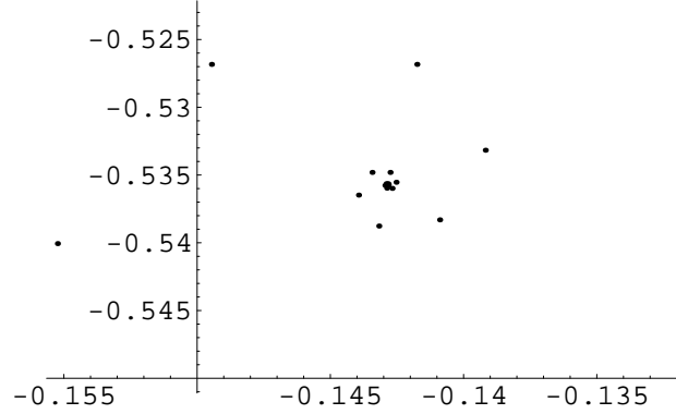
Figure 2: Expectation of \Xi_N in \mathcal{Cl}_{0,3} , 1 \leq N \leq 32 .
