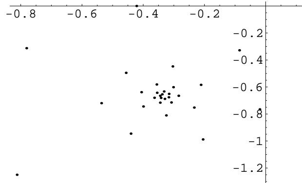
Figure 3: Expectation of \Xi_N in \mathcal{Cl}_{0,2} , 1 \leq N \leq 32 .
