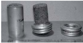
Figure 2. Shape histories of the tubes tested experimentally.
