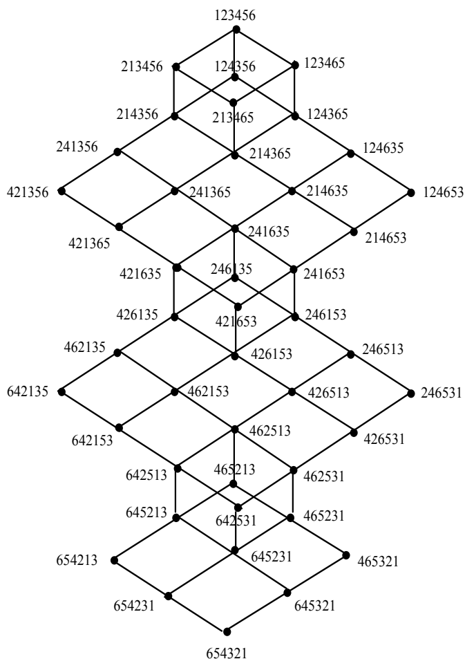
FIGURE 3 The distributive lattice AS(6)
